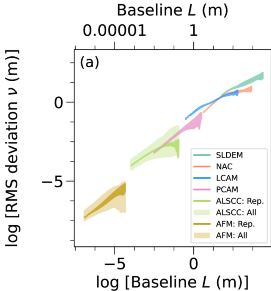
Figure 10. from Jun Du et al 2026 Astron. J. 171 doi:10.3847/1538-3881/ae6333 https://dx.doi.org/10.3847/1538-3881/ae6333 © 2026. The Author(s). Published by the American Astronomical Society.
