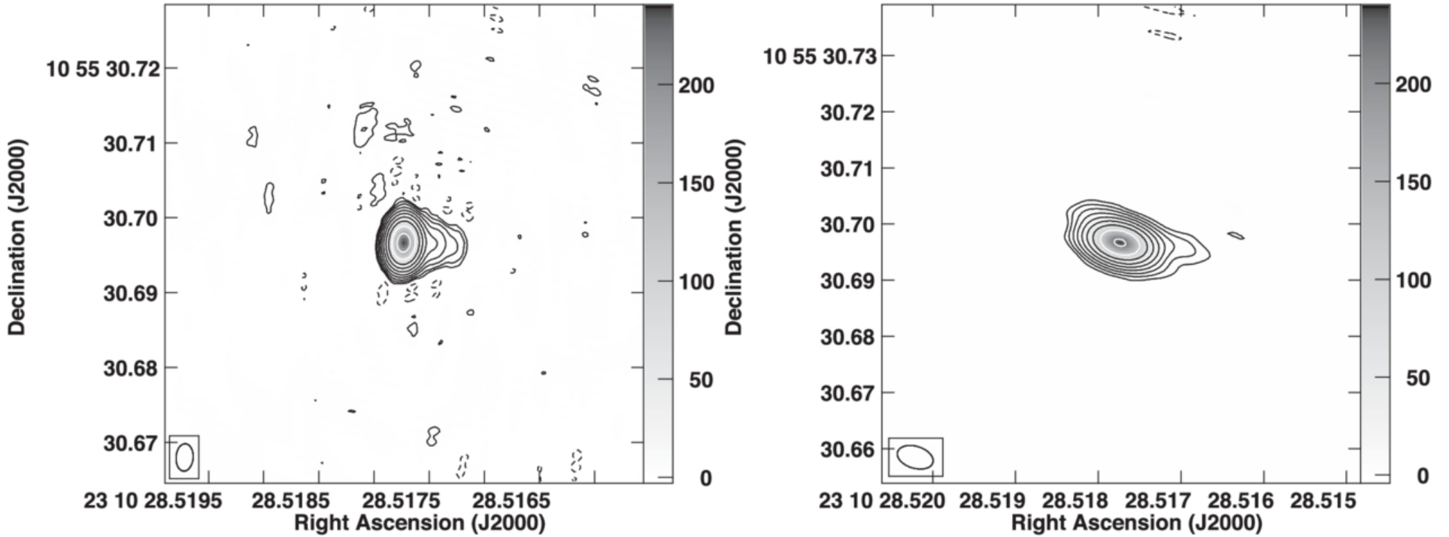
Figure 8. from Seppo Laine et al 2026 Astron. J. 171 doi:10.3847/1538-3881/ae61a2 https://dx.doi.org/10.3847/1538-3881/ae61a2 © 2026. The Author(s). Published by the American Astronomical Society.
