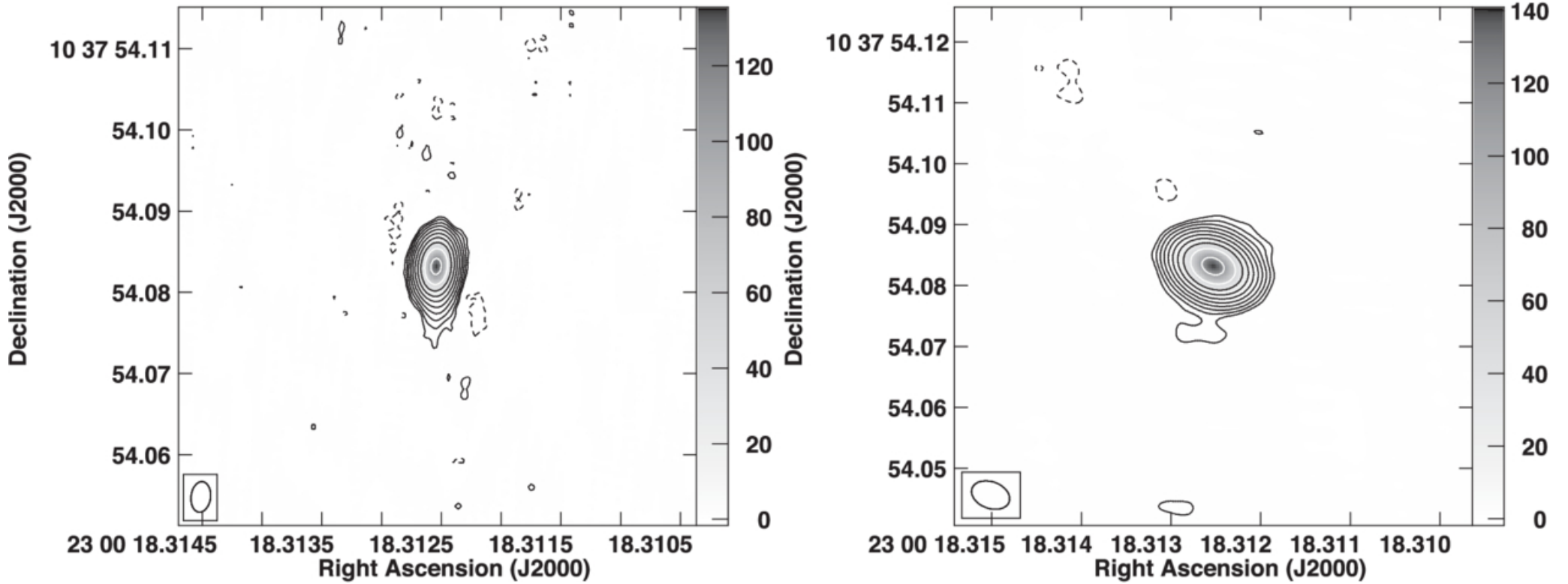
Figure 7. from Seppo Laine et al 2026 Astron. J. 171 doi:10.3847/1538-3881/ae61a2 https://dx.doi.org/10.3847/1538-3881/ae61a2 © 2026. The Author(s). Published by the American Astronomical Society.
