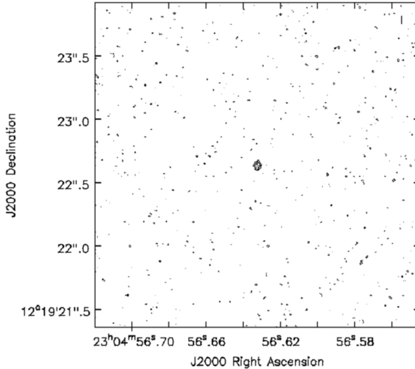
Figure 5. from Seppo Laine et al 2026 Astron. J. 171 doi:10.3847/1538-3881/ae61a2 https://dx.doi.org/10.3847/1538-3881/ae61a2 © 2026. The Author(s). Published by the American Astronomical Society.
