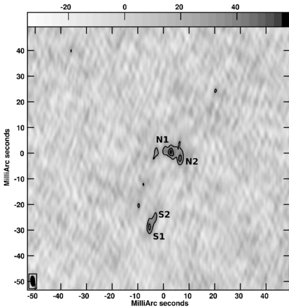
Figure 3. from Seppo Laine et al 2026 Astron. J. 171 doi:10.3847/1538-3881/ae61a2 https://dx.doi.org/10.3847/1538-3881/ae61a2 © 2026. The Author(s). Published by the American Astronomical Society.
