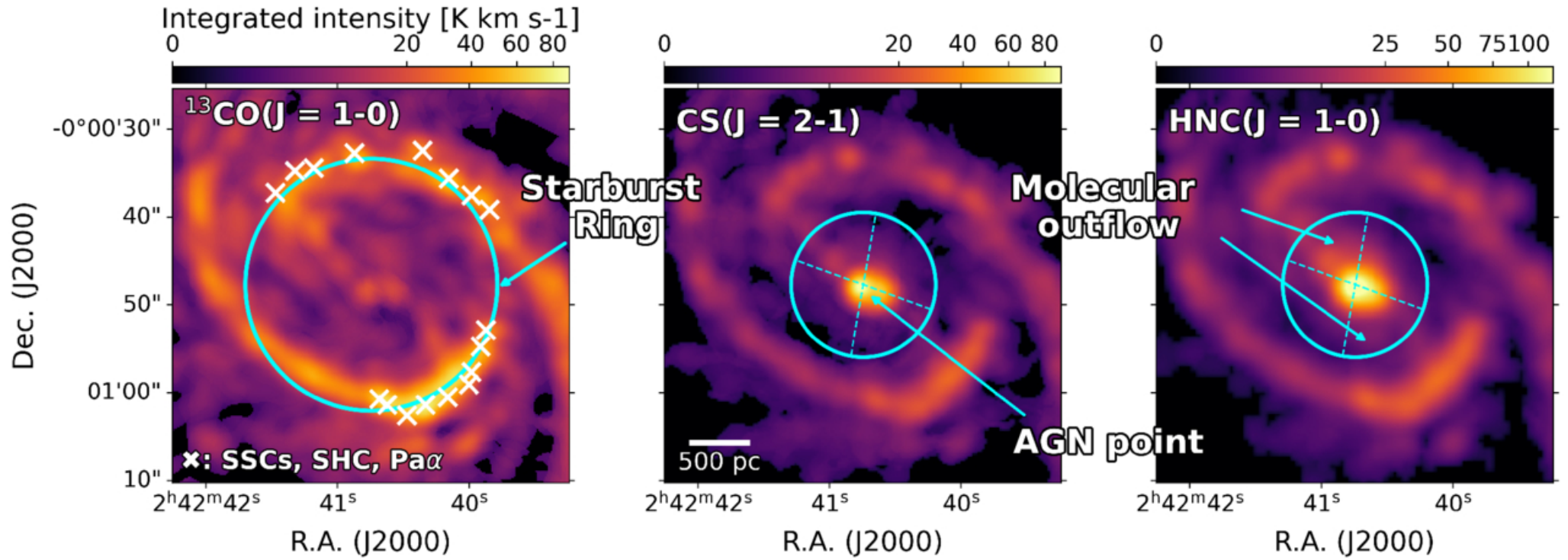
Figure 1. from Hiroma Okubo et al 2026 Astron. J. 172 doi:10.3847/1538-3881/ae6079 https://dx.doi.org/10.3847/1538-3881/ae6079 © 2026. The Author(s). Published by the American Astronomical Society.
