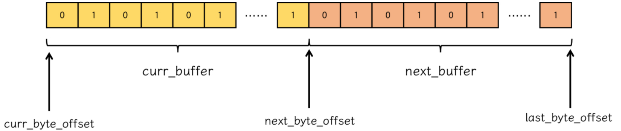
Figure 8. from Ya-Zhou Zhang et al 2026 Astron. J. 171 doi:10.3847/1538-3881/ae6066 https://dx.doi.org/10.3847/1538-3881/ae6066 © 2026. The Author(s). Published by the American Astronomical Society.
