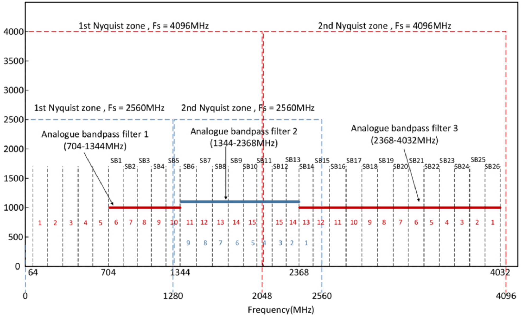
Figure 2. from Ya-Zhou Zhang et al 2026 Astron. J. 171 doi:10.3847/1538-3881/ae6066 https://dx.doi.org/10.3847/1538-3881/ae6066 © 2026. The Author(s). Published by the American Astronomical Society.
