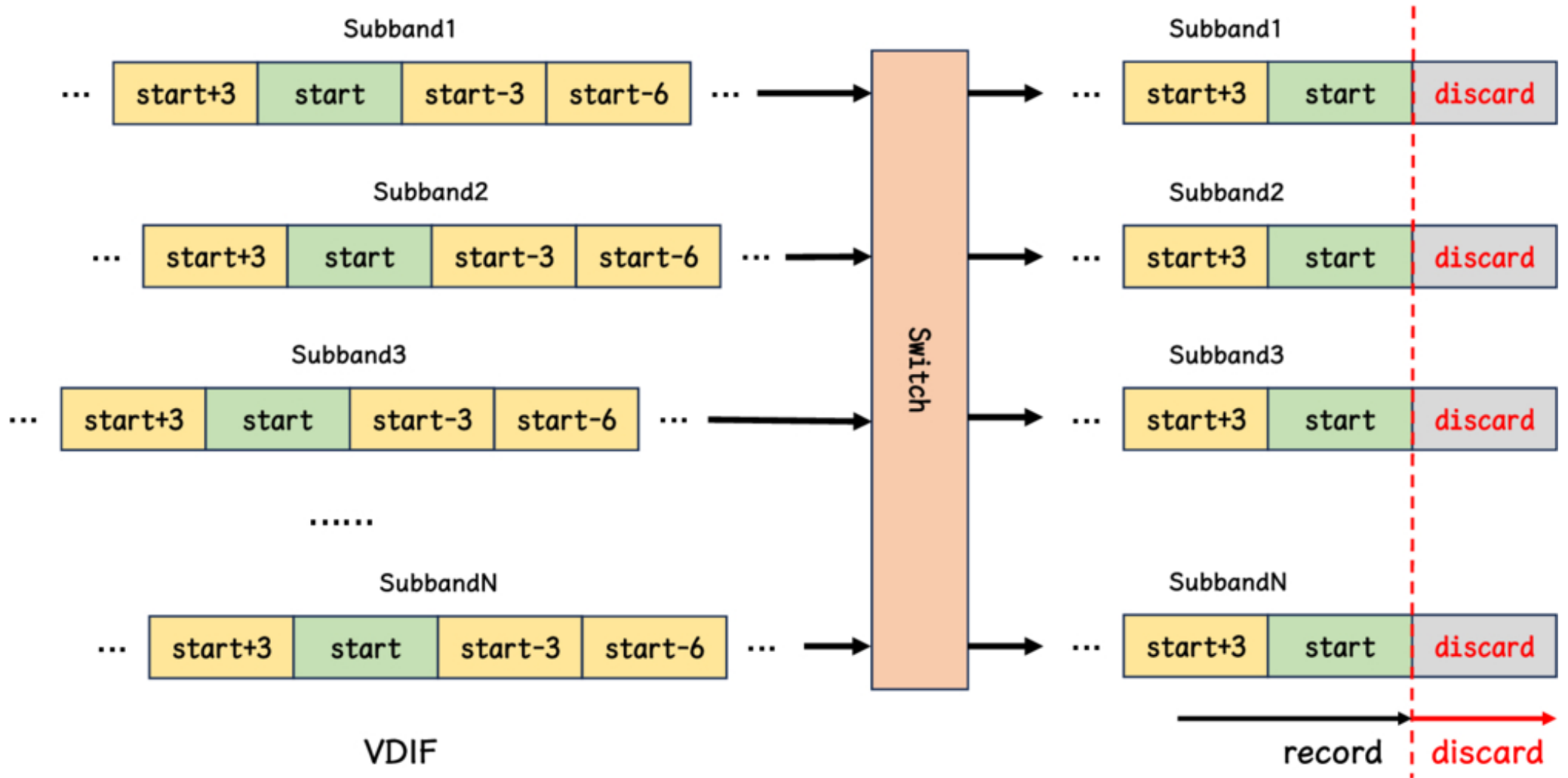
Figure 14. from Ya-Zhou Zhang et al 2026 Astron. J. 171 doi:10.3847/1538-3881/ae6066 https://dx.doi.org/10.3847/1538-3881/ae6066 © 2026. The Author(s). Published by the American Astronomical Society.
