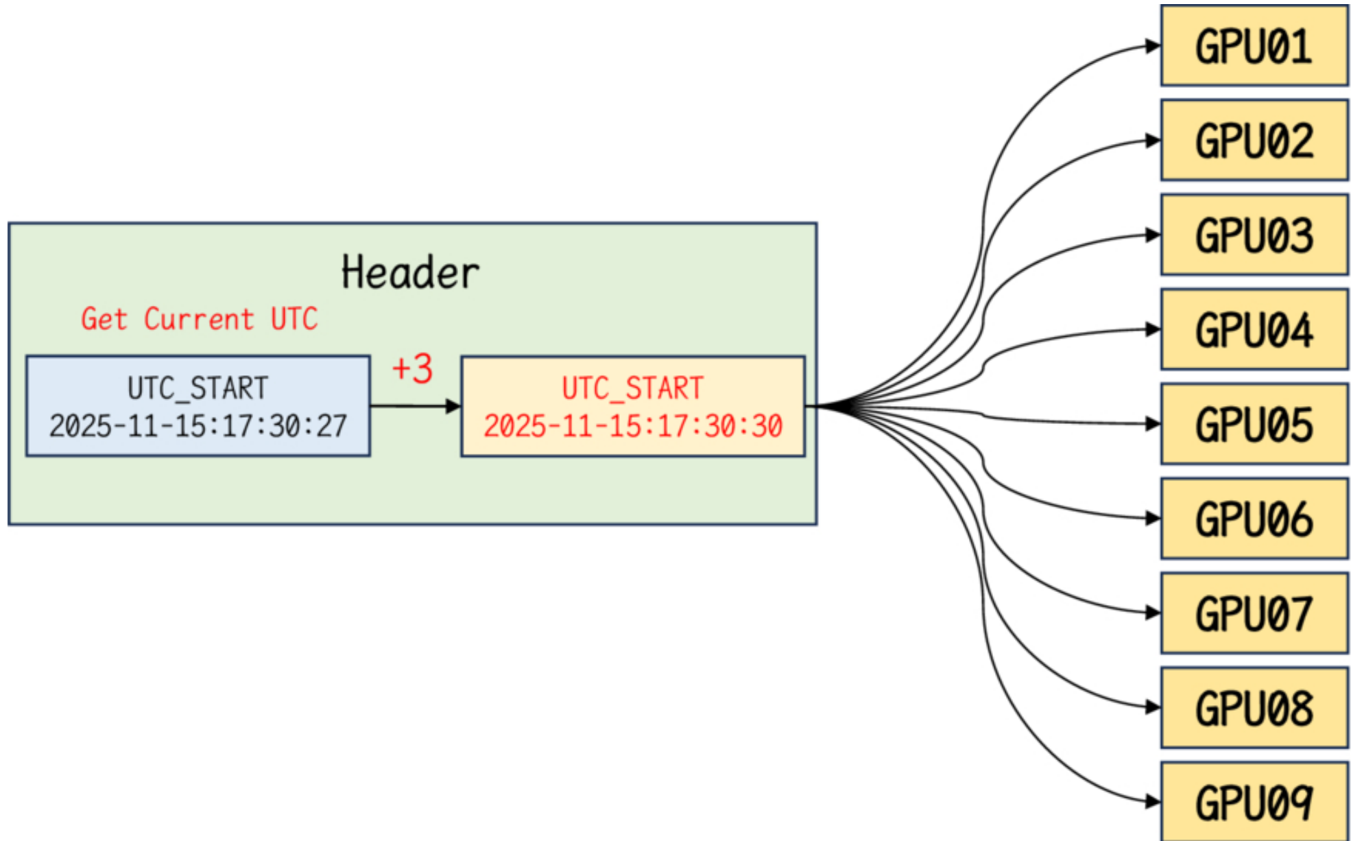
Figure 13. from Ya-Zhou Zhang et al 2026 Astron. J. 171 doi:10.3847/1538-3881/ae6066 https://dx.doi.org/10.3847/1538-3881/ae6066 © 2026. The Author(s). Published by the American Astronomical Society.
