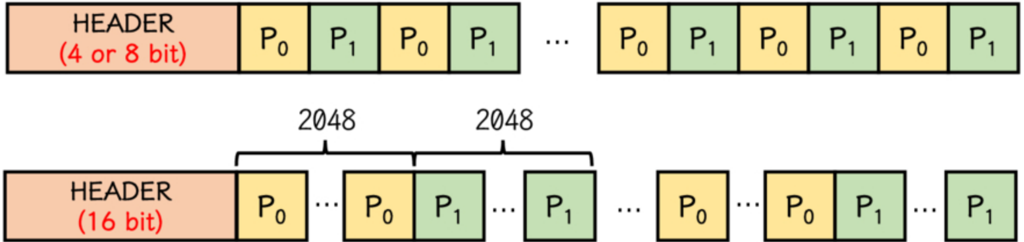
Figure 12. from Ya-Zhou Zhang et al 2026 Astron. J. 171 doi:10.3847/1538-3881/ae6066 https://dx.doi.org/10.3847/1538-3881/ae6066 © 2026. The Author(s). Published by the American Astronomical Society.
