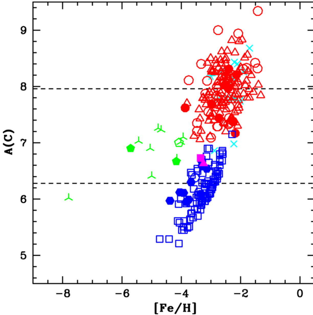
Figure 7. from Meenakshi Purandardas 2026 Astron. J. 171 doi:10.3847/1538-3881/ae5f93 https://dx.doi.org/10.3847/1538-3881/ae5f93 © 2026. The Author(s). Published by the American Astronomical Society.
