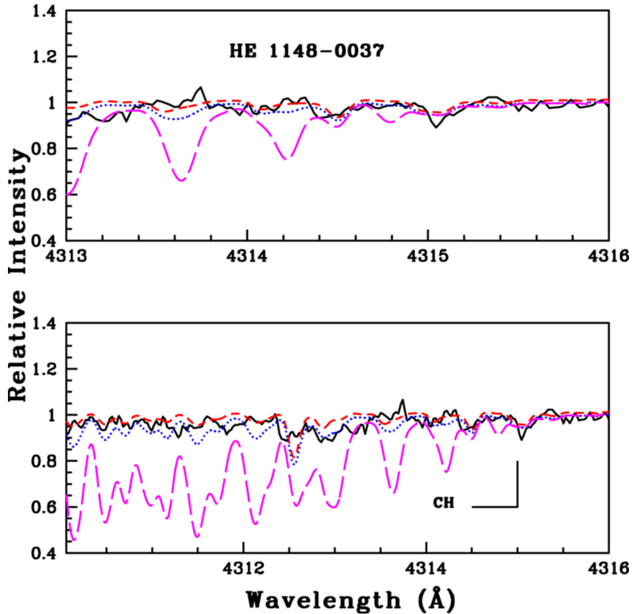
Figure 5. from Meenakshi Purandardas 2026 Astron. J. 171 doi:10.3847/1538-3881/ae5f93 https://dx.doi.org/10.3847/1538-3881/ae5f93 © 2026. The Author(s). Published by the American Astronomical Society.
