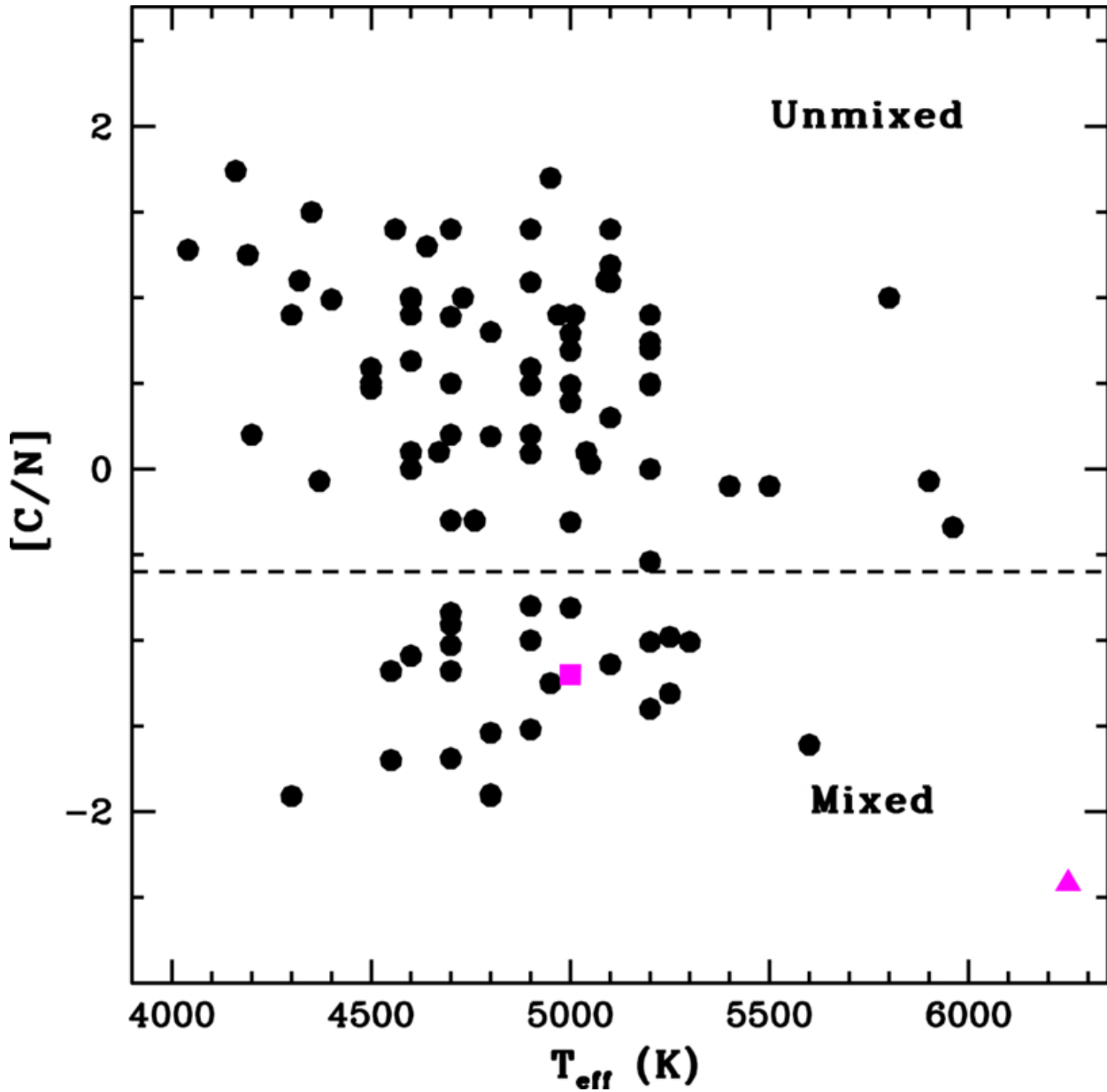
Figure 10. from Meenakshi Purandardas 2026 Astron. J. 171 doi:10.3847/1538-3881/ae5f93 https://dx.doi.org/10.3847/1538-3881/ae5f93 © 2026. The Author(s). Published by the American Astronomical Society.
