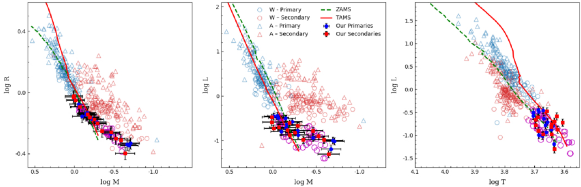
Figure 8. from A. Panchal and Kai Li 2026 Astron. J. 171 doi:10.3847/1538-3881/ae5f8f https://dx.doi.org/10.3847/1538-3881/ae5f8f © 2026. The Author(s). Published by the American Astronomical Society.
