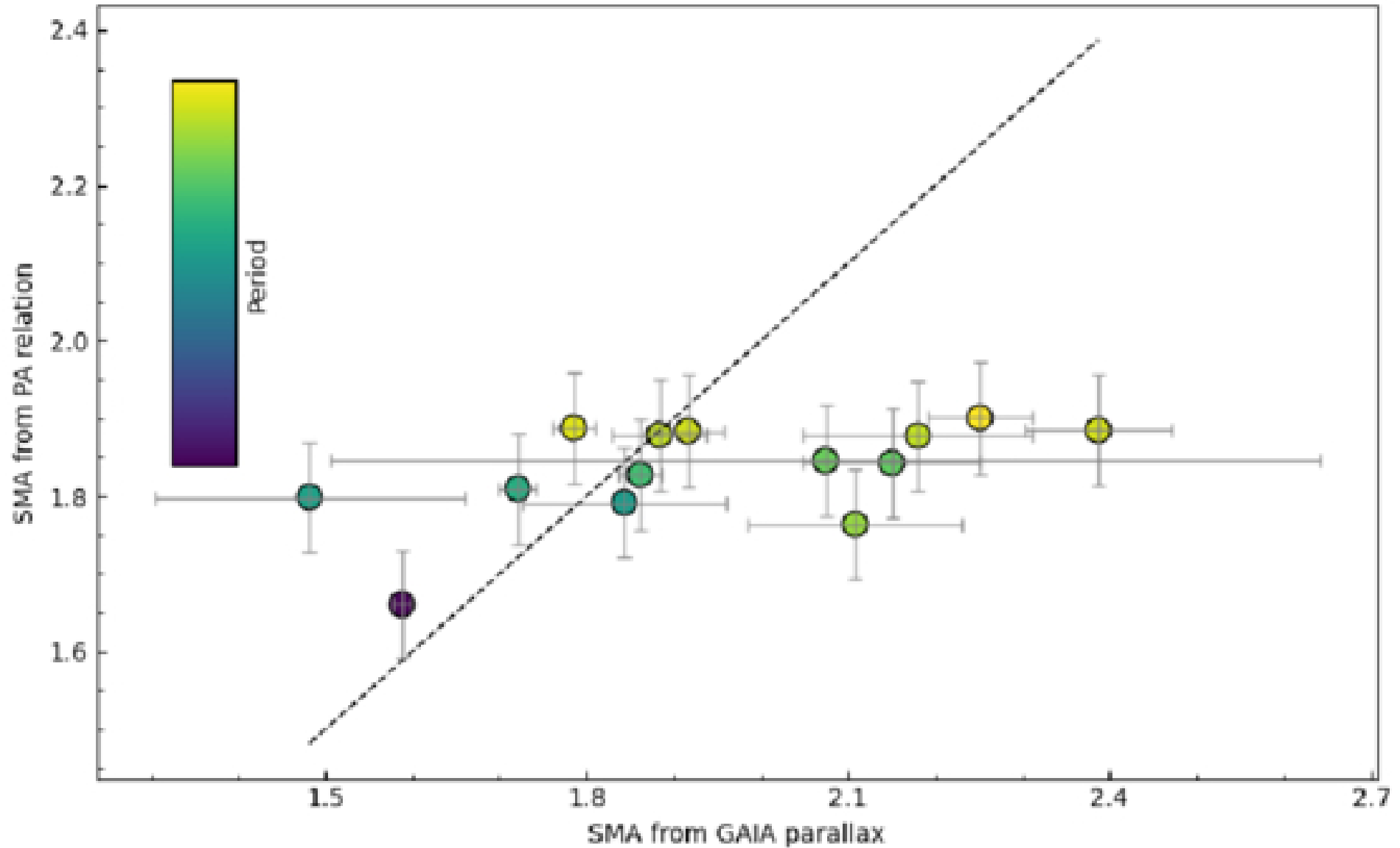
Figure 6. from A. Panchal and Kai Li 2026 Astron. J. 171 doi:10.3847/1538-3881/ae5f8f https://dx.doi.org/10.3847/1538-3881/ae5f8f © 2026. The Author(s). Published by the American Astronomical Society.
