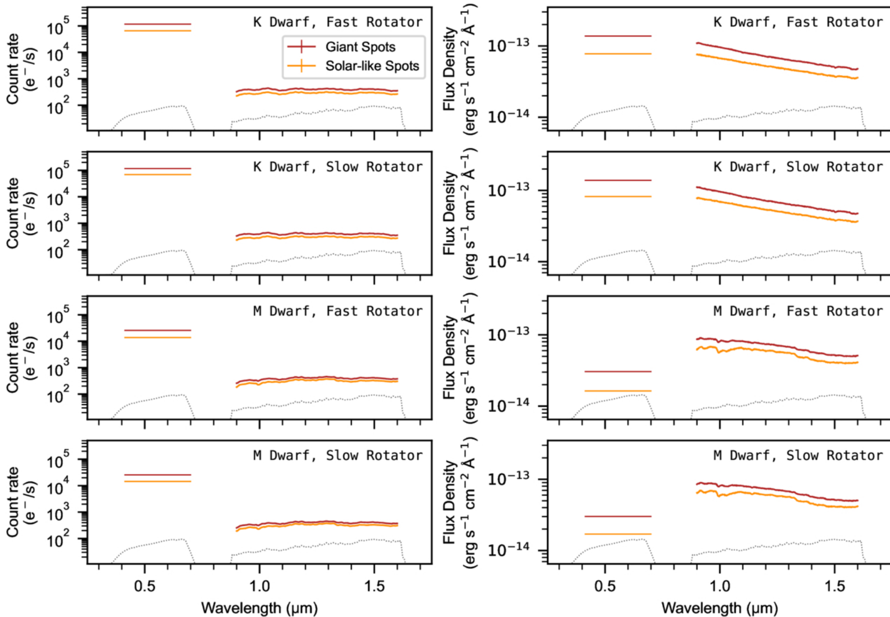
Figure 2. from Benjamin V. Rackham et al 2026 Astron. J. 171 doi:10.3847/1538-3881/ae5f63 https://dx.doi.org/10.3847/1538-3881/ae5f63 © 2026. The Author(s). Published by the American Astronomical Society.
