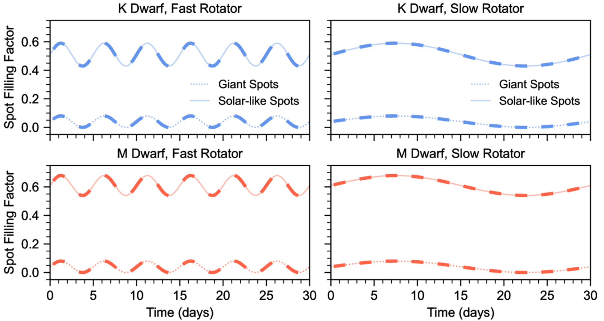
Figure 1. from Benjamin V. Rackham et al 2026 Astron. J. 171 doi:10.3847/1538-3881/ae5f63 https://dx.doi.org/10.3847/1538-3881/ae5f63 © 2026. The Author(s). Published by the American Astronomical Society.
