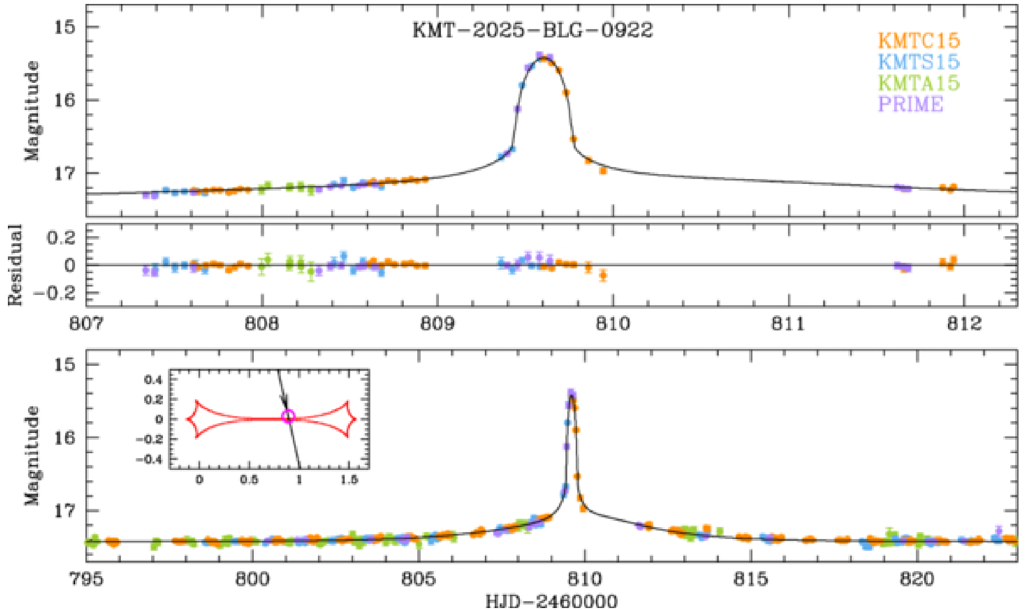
Figure 8. from Cheongho Han et al 2026 Astron. J. 171 doi:10.3847/1538-3881/ae5e5d https://dx.doi.org/10.3847/1538-3881/ae5e5d © 2026. The Author(s). Published by the American Astronomical Society.
