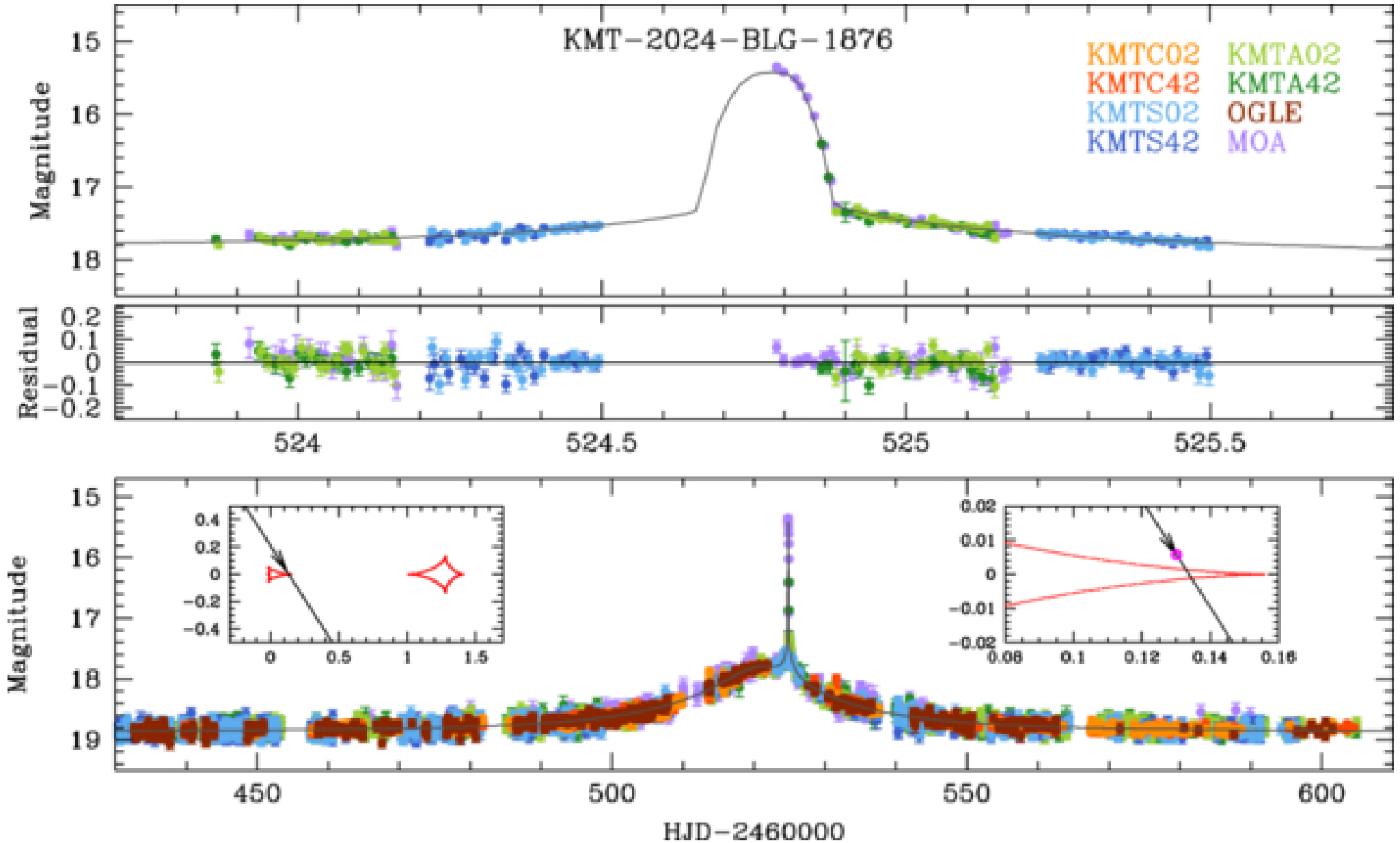
Figure 6. from Cheongho Han et al 2026 Astron. J. 171 doi:10.3847/1538-3881/ae5e5d https://dx.doi.org/10.3847/1538-3881/ae5e5d © 2026. The Author(s). Published by the American Astronomical Society.
