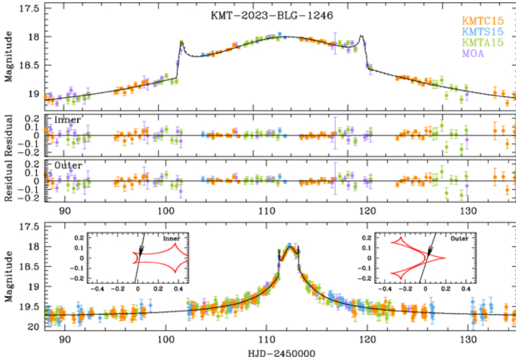
Figure 2. from Cheongho Han et al 2026 Astron. J. 171 doi:10.3847/1538-3881/ae5e5d https://dx.doi.org/10.3847/1538-3881/ae5e5d © 2026. The Author(s). Published by the American Astronomical Society.
