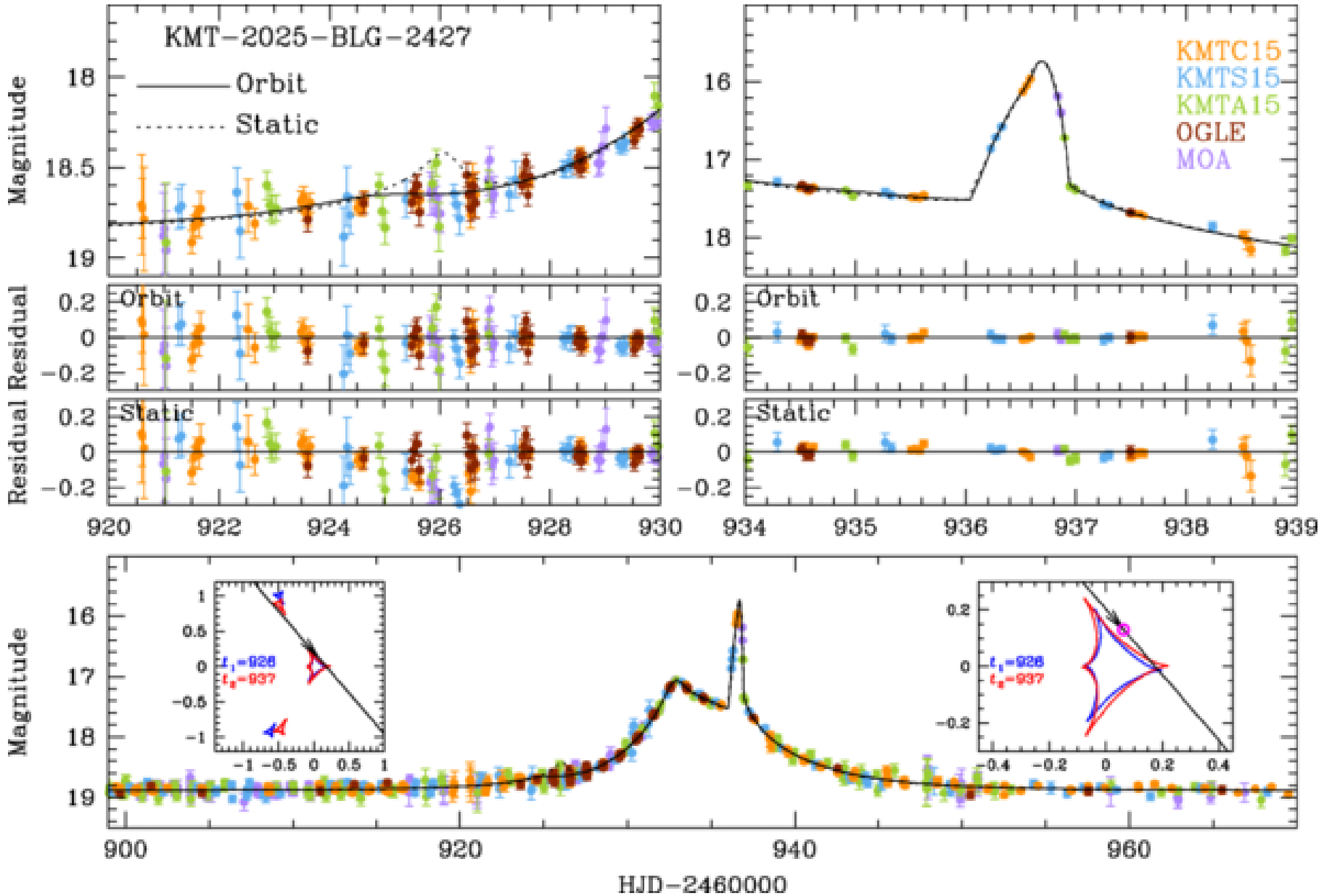
Figure 10. from Cheongho Han et al 2026 Astron. J. 171 doi:10.3847/1538-3881/ae5e5d https://dx.doi.org/10.3847/1538-3881/ae5e5d © 2026. The Author(s). Published by the American Astronomical Society.
