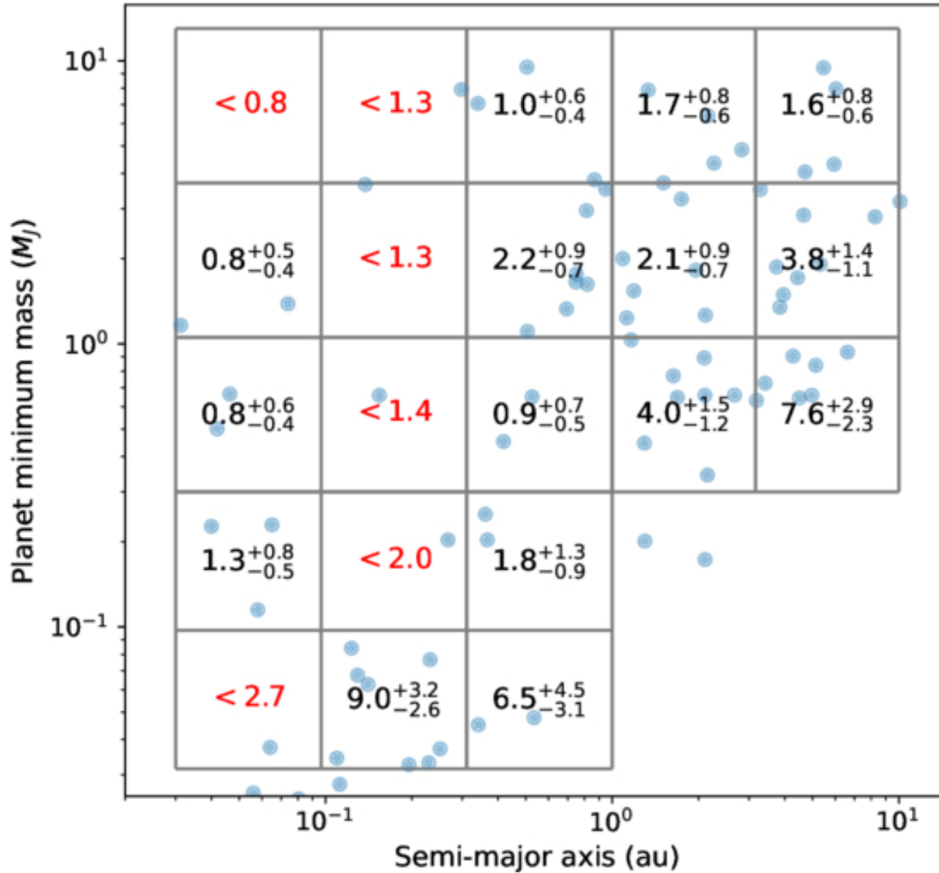
Figure 4. from Jiayin Li et al 2026 Astron. J. 172 doi:10.3847/1538-3881/ae5e52 https://dx.doi.org/10.3847/1538-3881/ae5e52 © 2026. The Author(s). Published by the American Astronomical Society.
