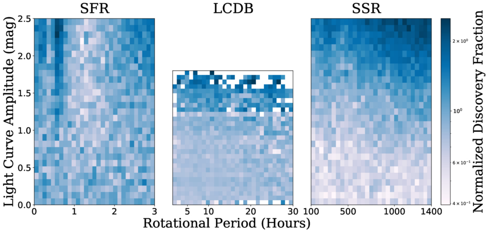
Figure 7. from Alexander J. Fleming et al 2026 Astron. J. 171 doi:10.3847/1538-3881/ae5e49 https://dx.doi.org/10.3847/1538-3881/ae5e49 © 2026. The Author(s). Published by the American Astronomical Society.
