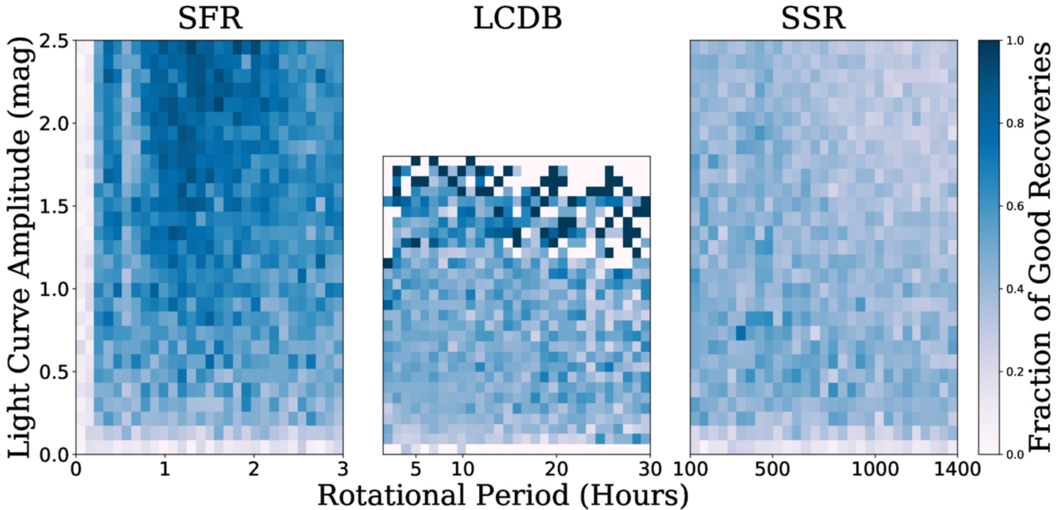
Figure 6. from Alexander J. Fleming et al 2026 Astron. J. 171 doi:10.3847/1538-3881/ae5e49 https://dx.doi.org/10.3847/1538-3881/ae5e49 © 2026. The Author(s). Published by the American Astronomical Society.
