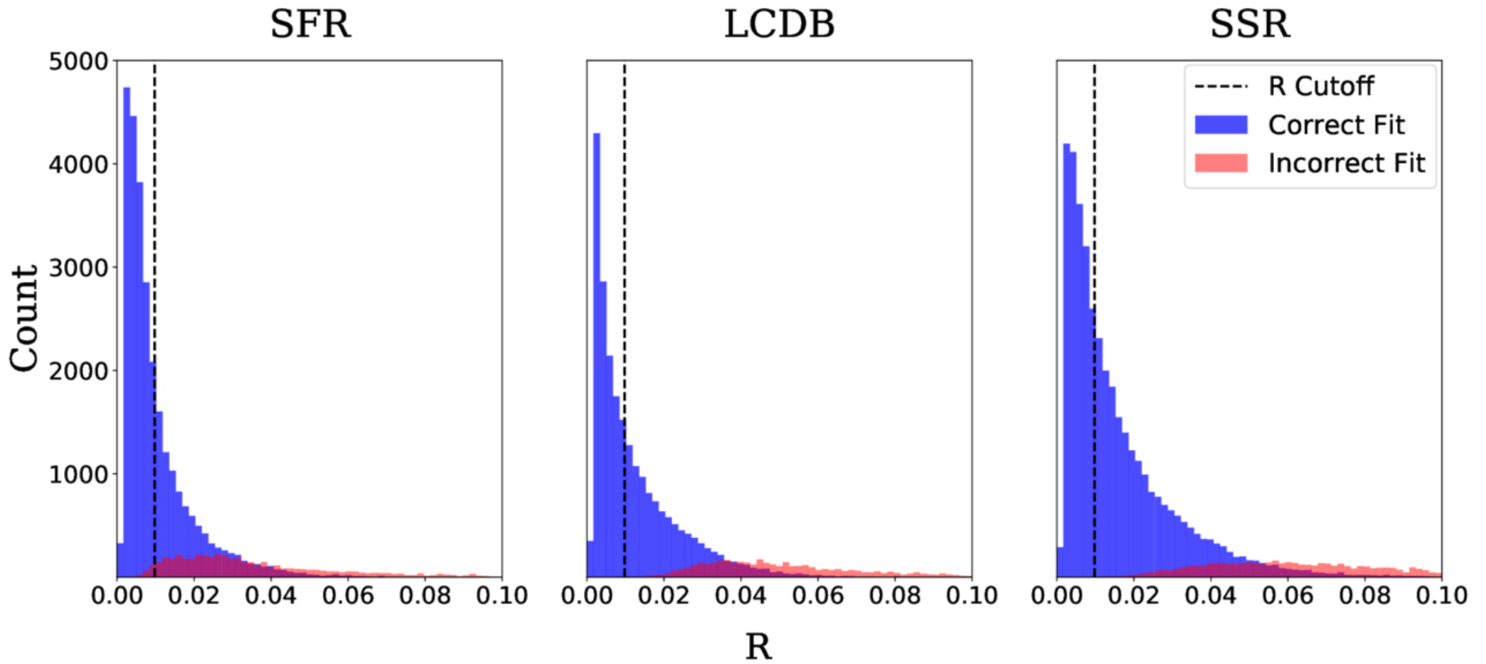
Figure 4. from Alexander J. Fleming et al 2026 Astron. J. 171 doi:10.3847/1538-3881/ae5e49 https://dx.doi.org/10.3847/1538-3881/ae5e49 © 2026. The Author(s). Published by the American Astronomical Society.
