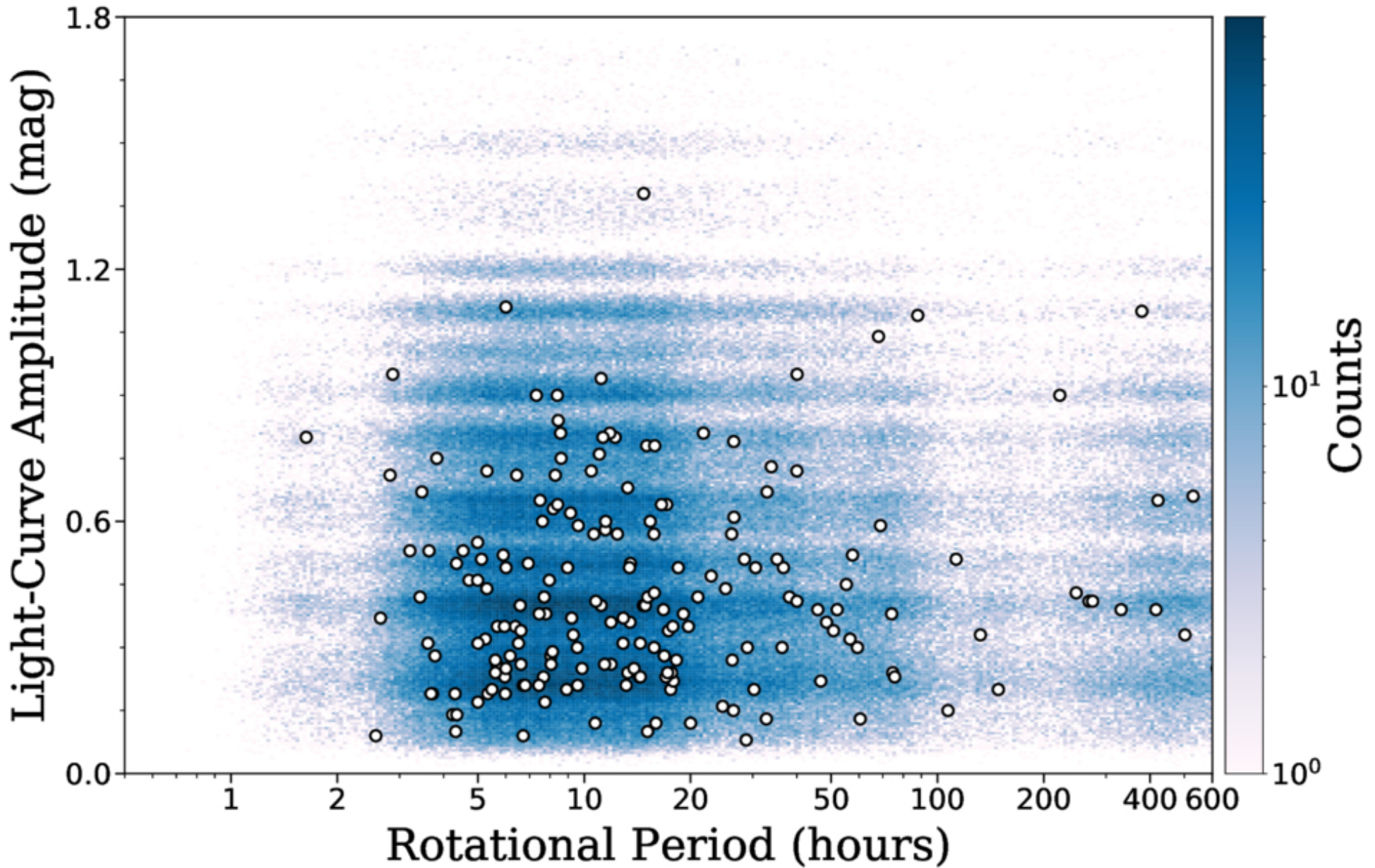
Figure 3. from Alexander J. Fleming et al 2026 Astron. J. 171 doi:10.3847/1538-3881/ae5e49 https://dx.doi.org/10.3847/1538-3881/ae5e49 © 2026. The Author(s). Published by the American Astronomical Society.
