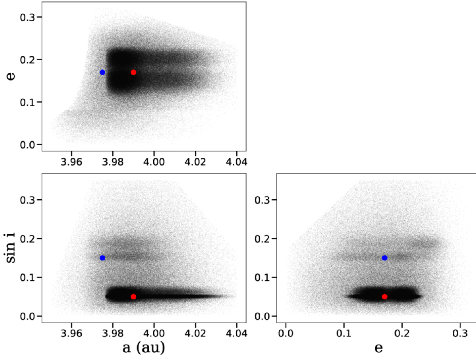
Figure 2. from Alexander J. Fleming et al 2026 Astron. J. 171 doi:10.3847/1538-3881/ae5e49 https://dx.doi.org/10.3847/1538-3881/ae5e49 © 2026. The Author(s). Published by the American Astronomical Society.
