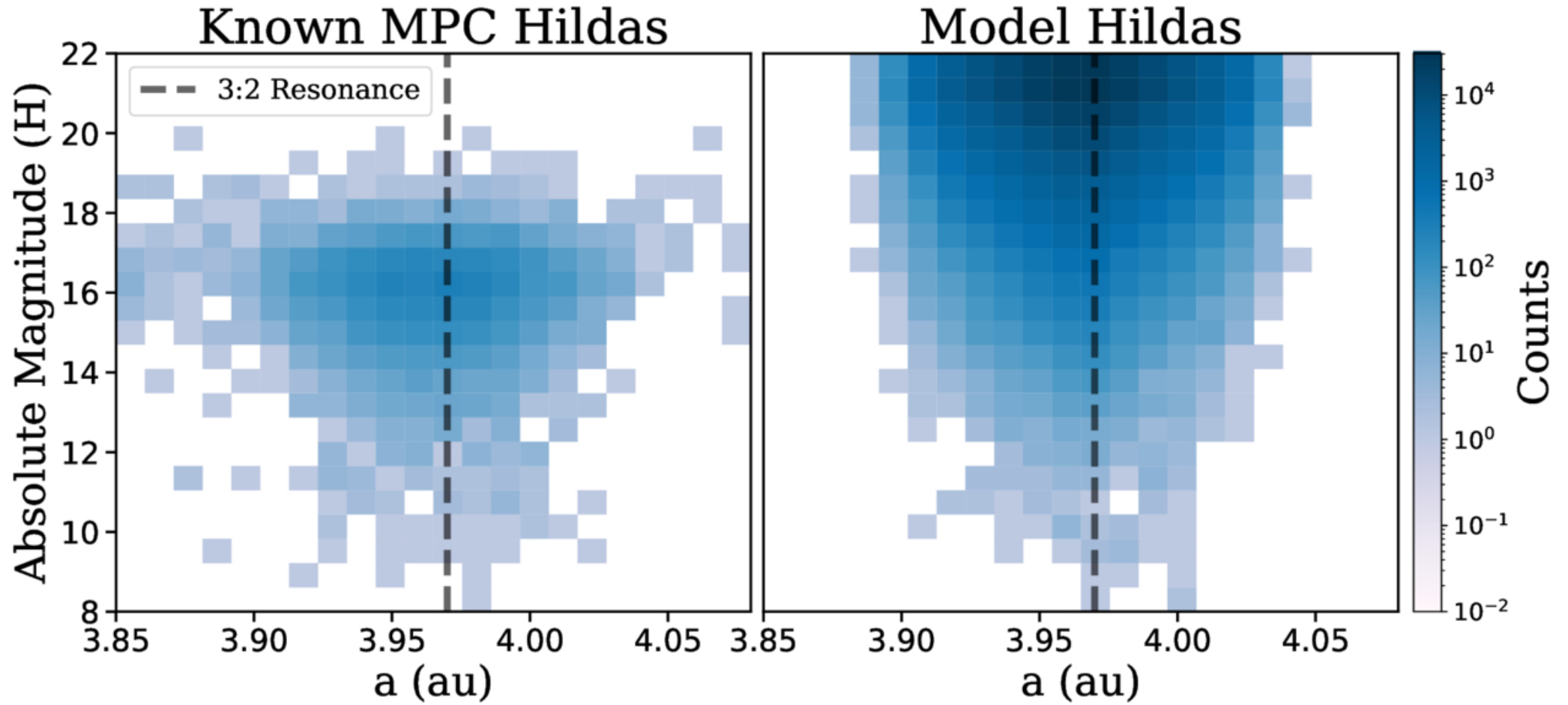
Figure 1. from Alexander J. Fleming et al 2026 Astron. J. 171 doi:10.3847/1538-3881/ae5e49 https://dx.doi.org/10.3847/1538-3881/ae5e49 © 2026. The Author(s). Published by the American Astronomical Society.
