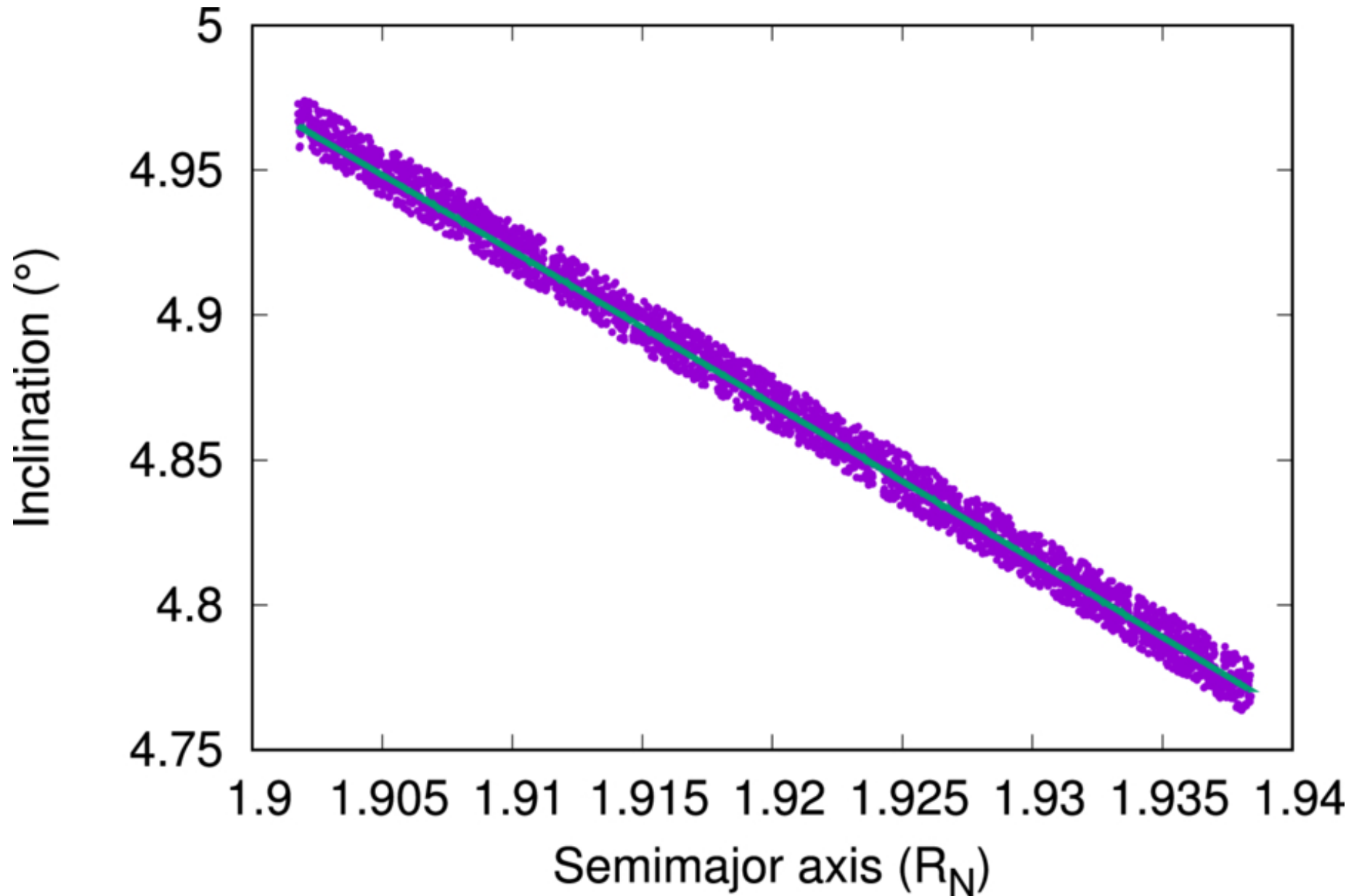
Figure 2. from Matija uk et al 2026 Astron. J. 171 doi:10.3847/1538-3881/ae5e47 https://dx.doi.org/10.3847/1538-3881/ae5e47 © 2026. The Author(s). Published by the American Astronomical Society.
