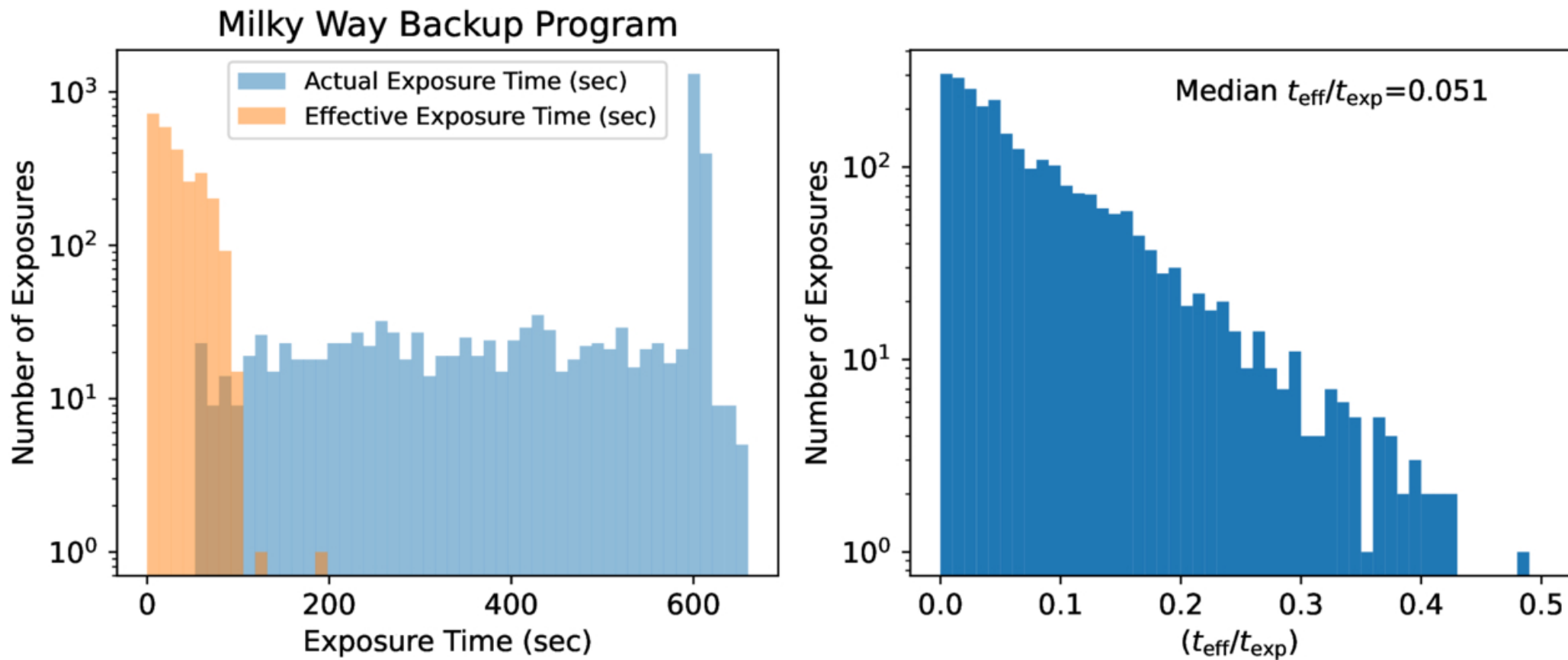
Figure 6. from Arjun Dey et al 2026 Astron. J. 171 doi:10.3847/1538-3881/ae5dd0 https://dx.doi.org/10.3847/1538-3881/ae5dd0 © 2026. The Author(s). Published by the American Astronomical Society.
