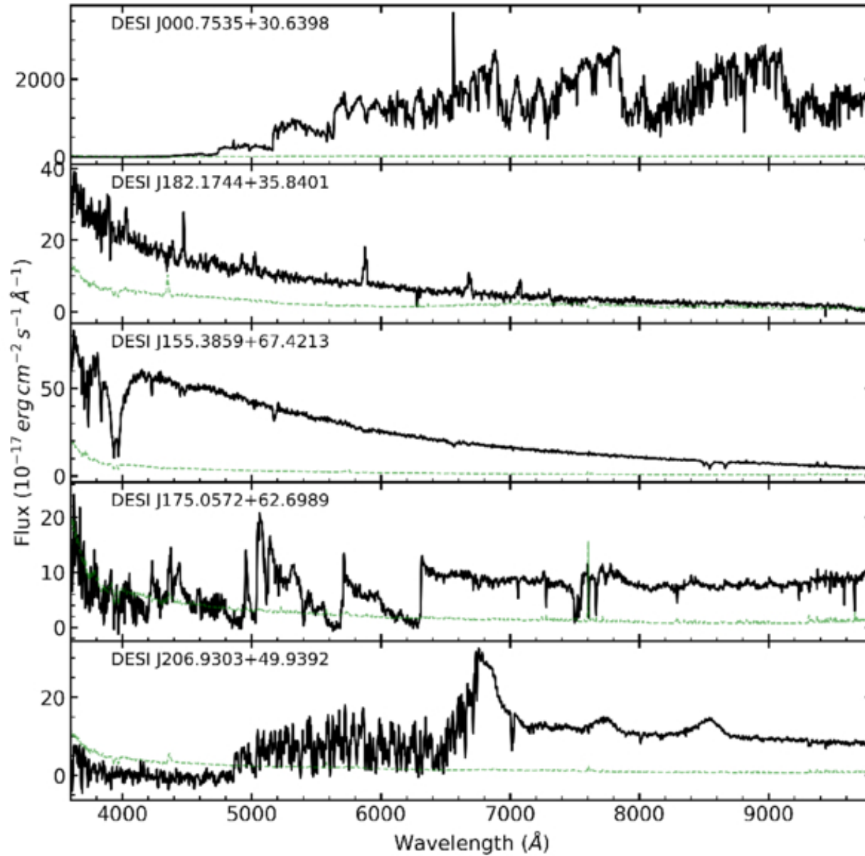
Figure 19. from Arjun Dey et al 2026 Astron. J. 171 doi:10.3847/1538-3881/ae5dd0 https://dx.doi.org/10.3847/1538-3881/ae5dd0 © 2026. The Author(s). Published by the American Astronomical Society.
