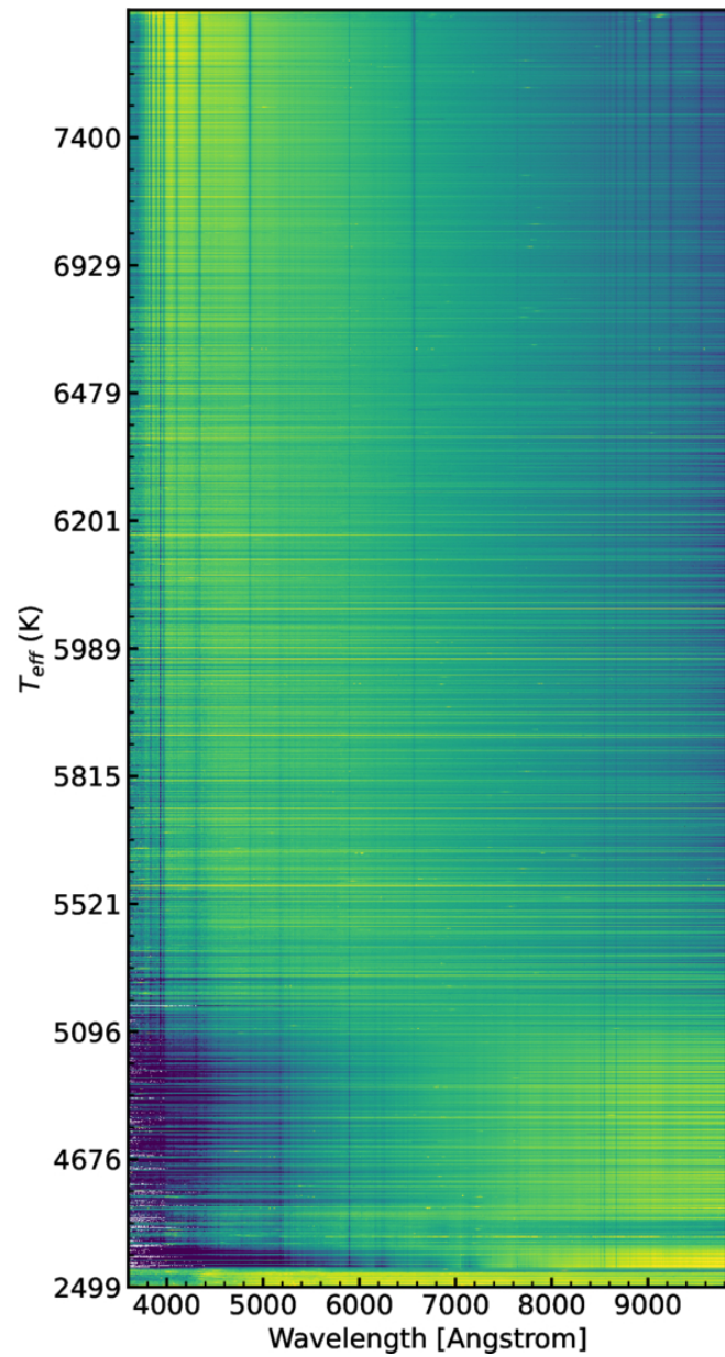
Figure 18. from Arjun Dey et al 2026 Astron. J. 171 doi:10.3847/1538-3881/ae5dd0 https://dx.doi.org/10.3847/1538-3881/ae5dd0 © 2026. The Author(s). Published by the American Astronomical Society.
