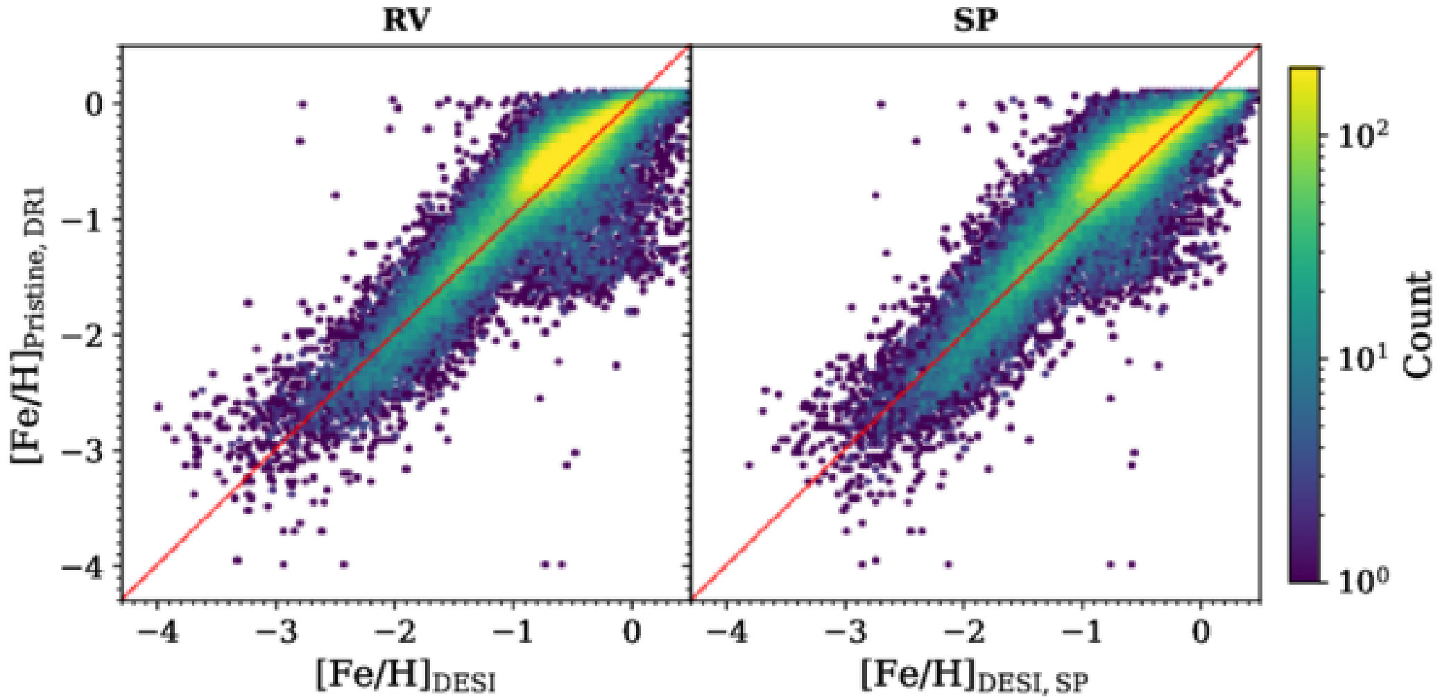
Figure 16. from Arjun Dey et al 2026 Astron. J. 171 doi:10.3847/1538-3881/ae5dd0 https://dx.doi.org/10.3847/1538-3881/ae5dd0 © 2026. The Author(s). Published by the American Astronomical Society.
