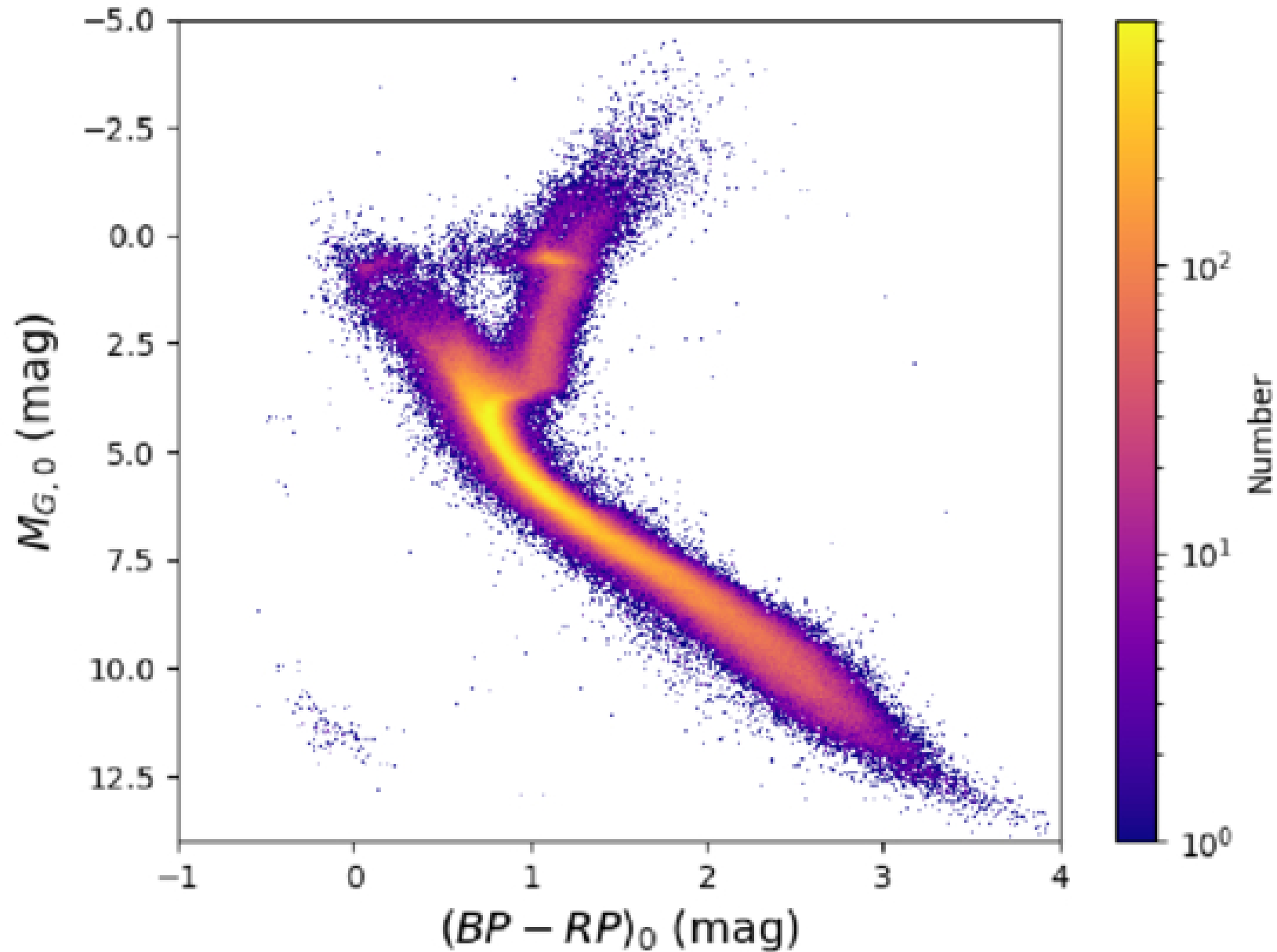
Figure 13. from Arjun Dey et al 2026 Astron. J. 171 doi:10.3847/1538-3881/ae5dd0 https://dx.doi.org/10.3847/1538-3881/ae5dd0 © 2026. The Author(s). Published by the American Astronomical Society.
