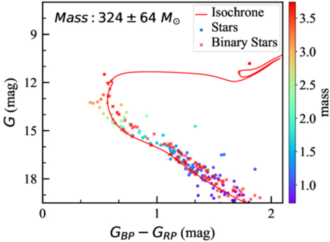
Figure 3. from Jing Chen et al 2026 Astron. J. 171 doi:10.3847/1538-3881/ae5d30 https://dx.doi.org/10.3847/1538-3881/ae5d30 © 2026. The Author(s). Published by the American Astronomical Society.
