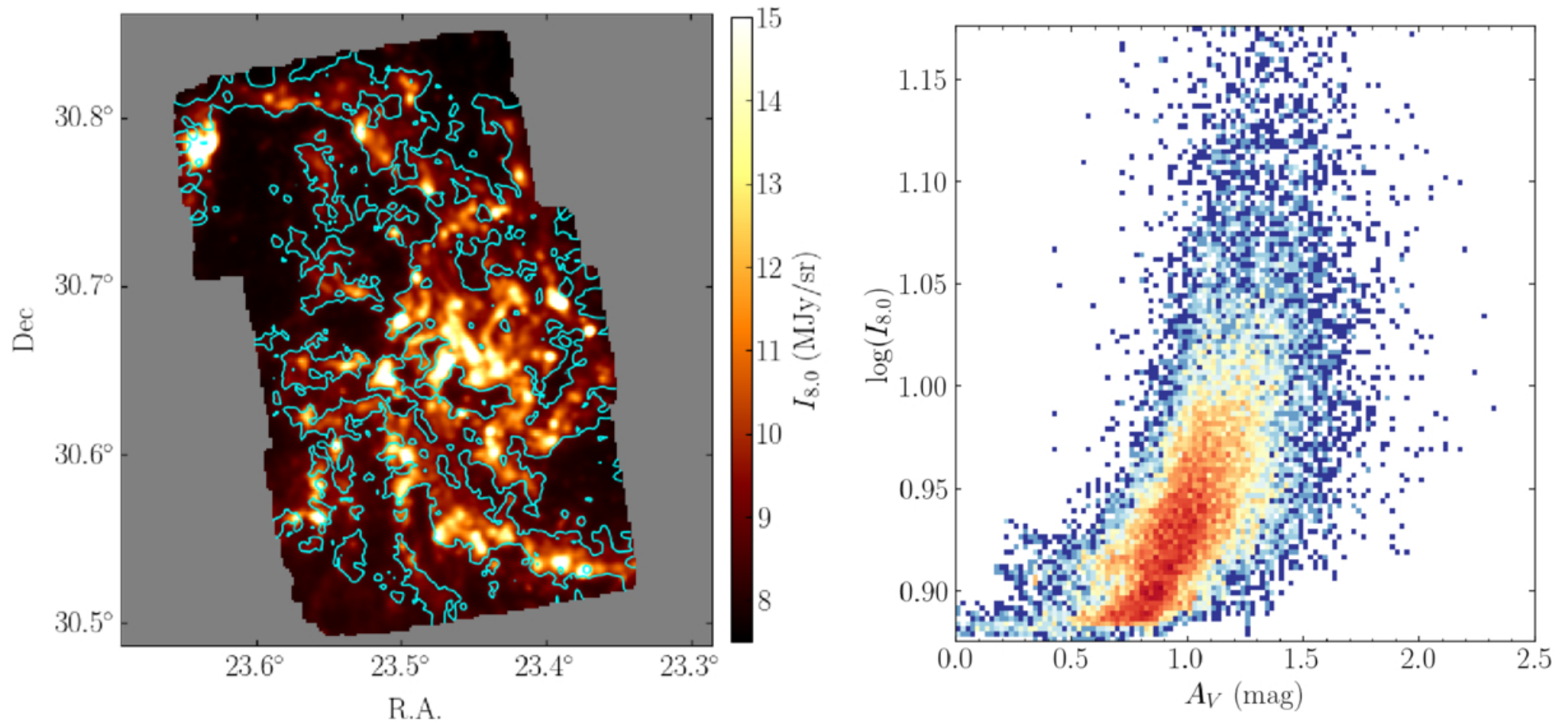
Figure 4. from Yuxi Wang et al 2026 Astron. J. 171 doi:10.3847/1538-3881/ae5bb5 https://dx.doi.org/10.3847/1538-3881/ae5bb5 © 2026. The Author(s). Published by the American Astronomical Society.
