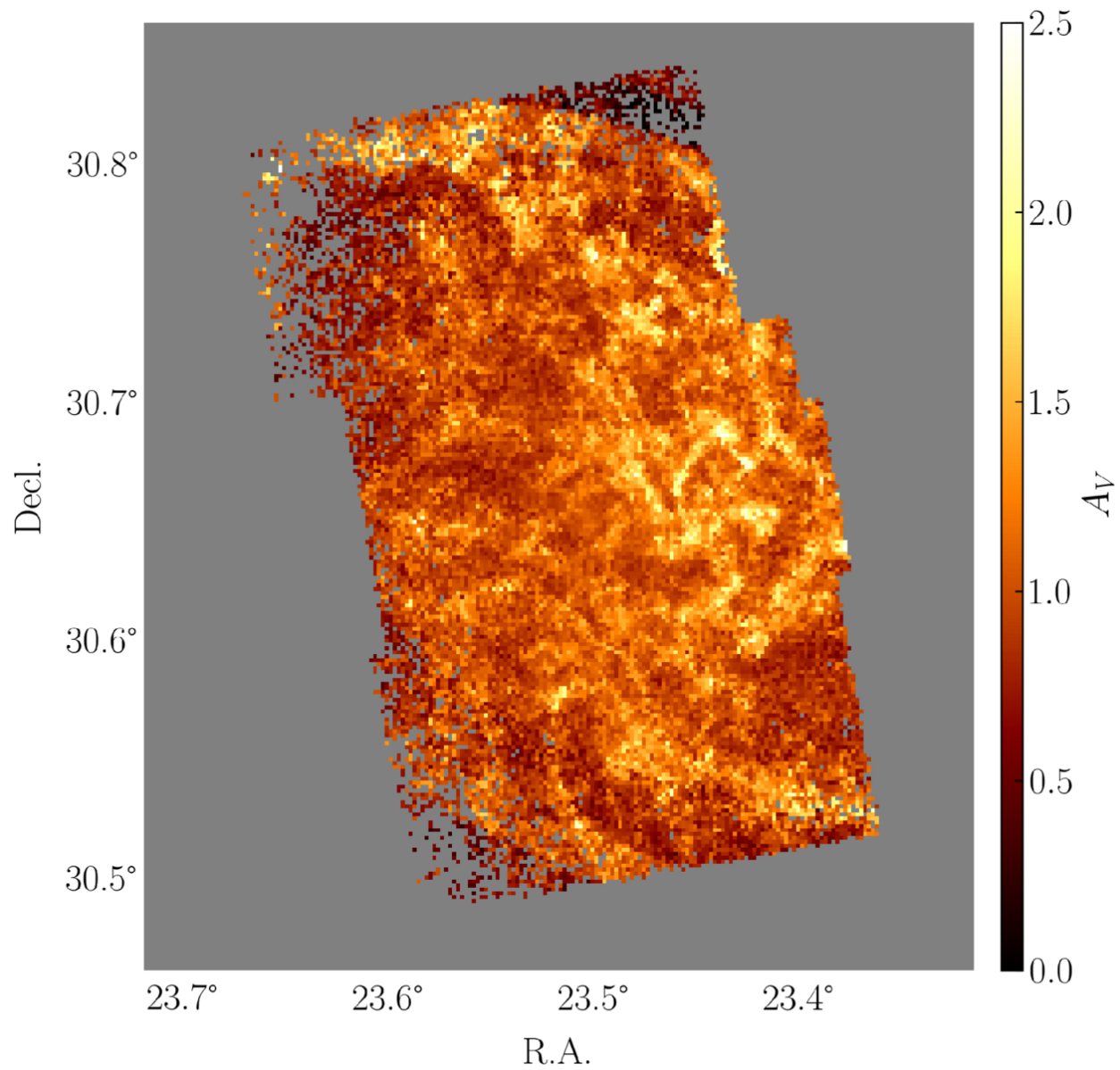
Figure 3. from Yuxi Wang et al 2026 Astron. J. 171 doi:10.3847/1538-3881/ae5bb5 https://dx.doi.org/10.3847/1538-3881/ae5bb5 © 2026. The Author(s). Published by the American Astronomical Society.
