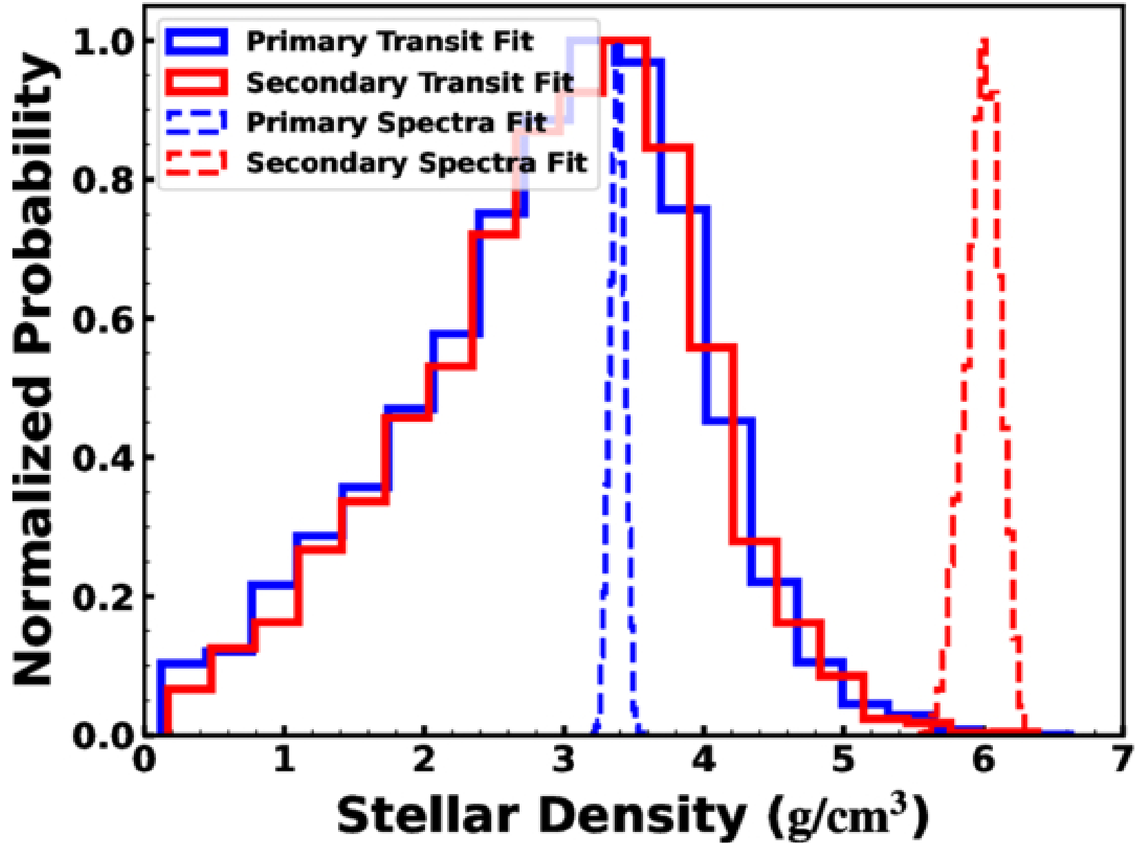
Figure 3. from Nathanael Burns-Watson et al 2026 Astron. J. 171 doi:10.3847/1538-3881/ae5ba4 https://dx.doi.org/10.3847/1538-3881/ae5ba4 © 2026. The Author(s). Published by the American Astronomical Society.
