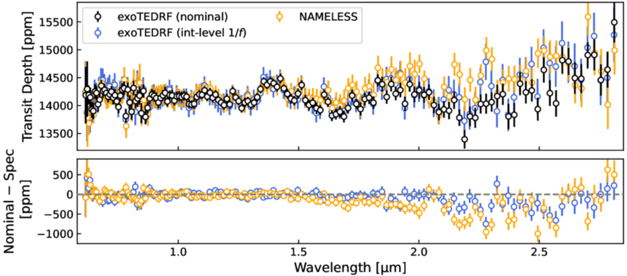
Figure 9. from Michael Radica et al 2026 Astron. J. 171 doi:10.3847/1538-3881/ae5b9f https://dx.doi.org/10.3847/1538-3881/ae5b9f © 2026. The Author(s). Published by the American Astronomical Society.
