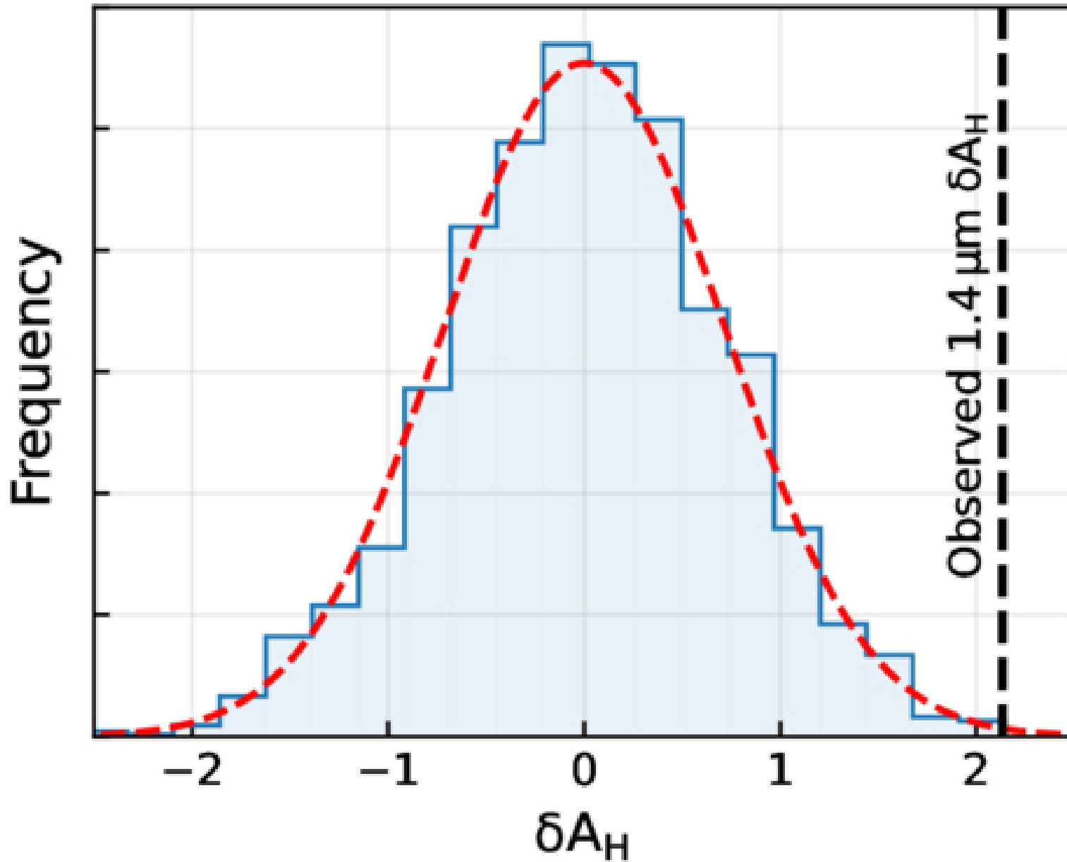
Figure 8. from Michael Radica et al 2026 Astron. J. 171 doi:10.3847/1538-3881/ae5b9f https://dx.doi.org/10.3847/1538-3881/ae5b9f © 2026. The Author(s). Published by the American Astronomical Society.
