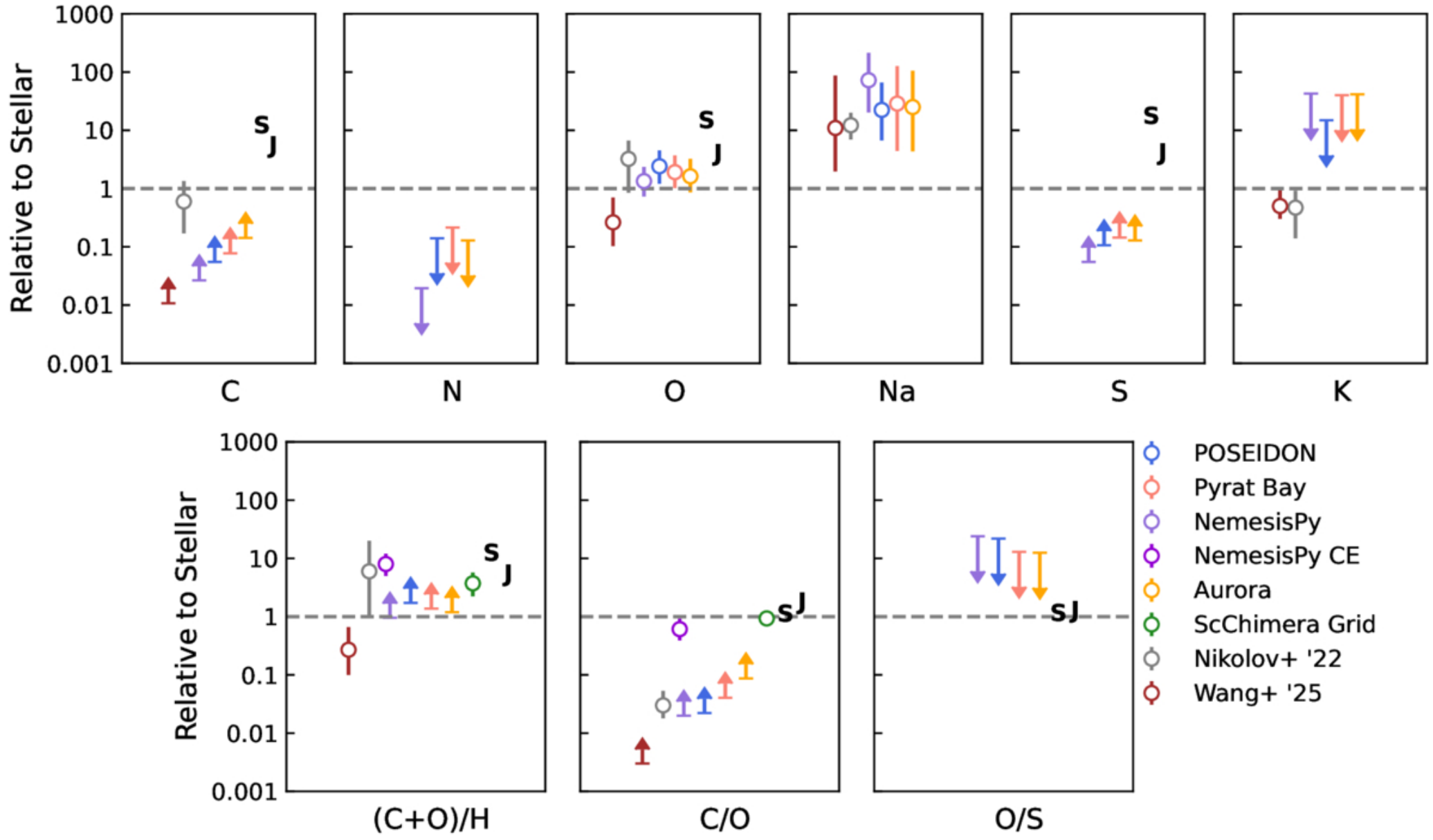
Figure 6. from Michael Radica et al 2026 Astron. J. 171 doi:10.3847/1538-3881/ae5b9f https://dx.doi.org/10.3847/1538-3881/ae5b9f © 2026. The Author(s). Published by the American Astronomical Society.
