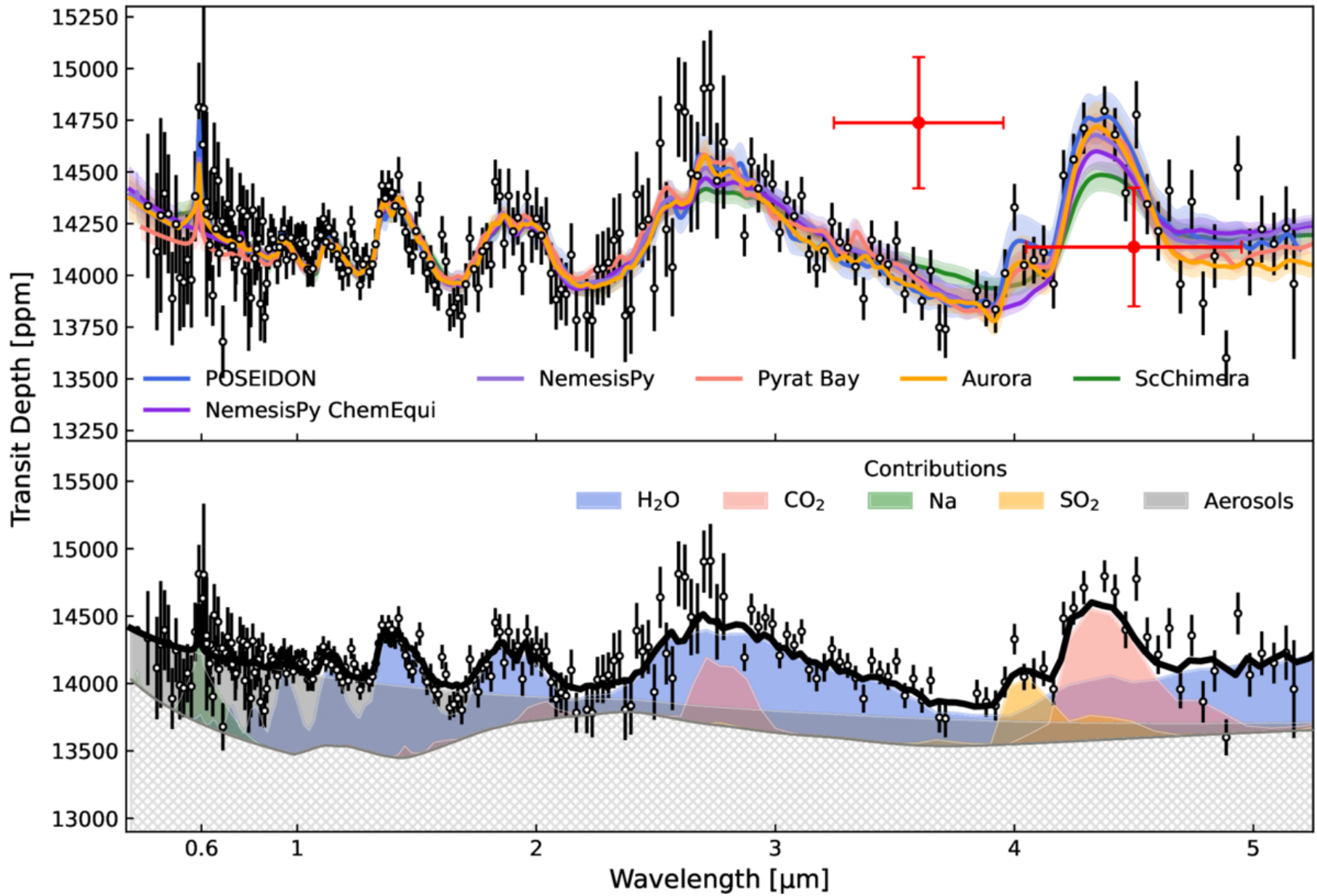
Figure 4. from Michael Radica et al 2026 Astron. J. 171 doi:10.3847/1538-3881/ae5b9f https://dx.doi.org/10.3847/1538-3881/ae5b9f © 2026. The Author(s). Published by the American Astronomical Society.
