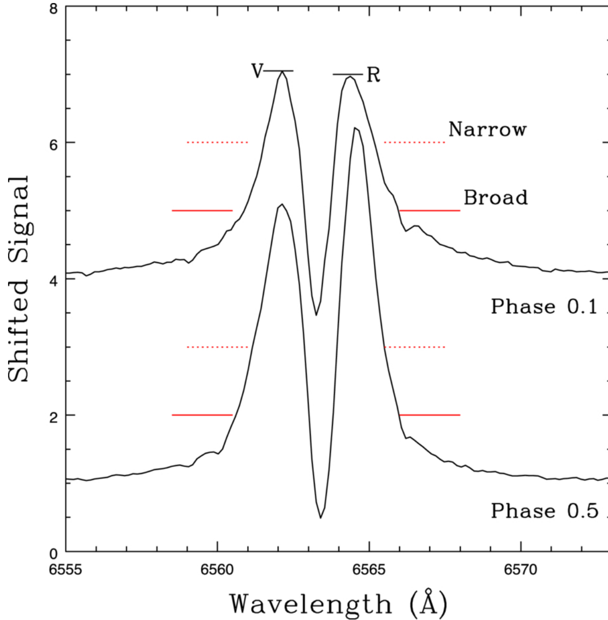
Figure 8. from T. J. Davidge 2026 Astron. J. 171 doi:10.3847/1538-3881/ae5b97 https://dx.doi.org/10.3847/1538-3881/ae5b97 © 2026. The Author(s). Published by the American Astronomical Society.
