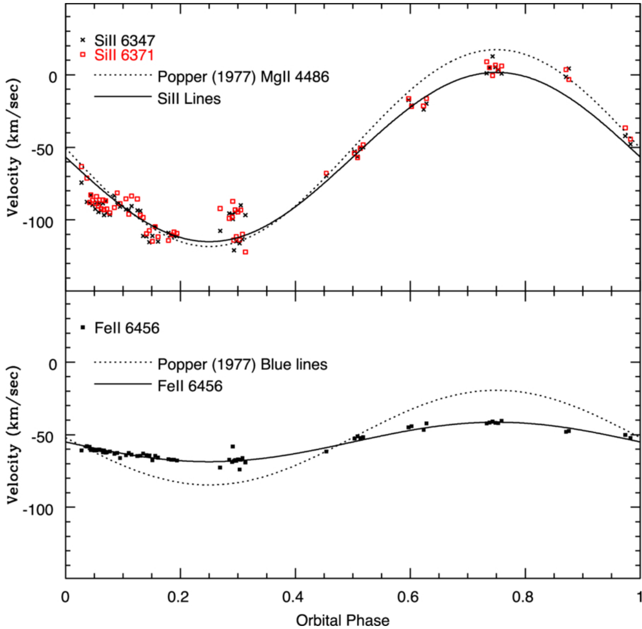
Figure 6. from T. J. Davidge 2026 Astron. J. 171 doi:10.3847/1538-3881/ae5b97 https://dx.doi.org/10.3847/1538-3881/ae5b97 © 2026. The Author(s). Published by the American Astronomical Society.
