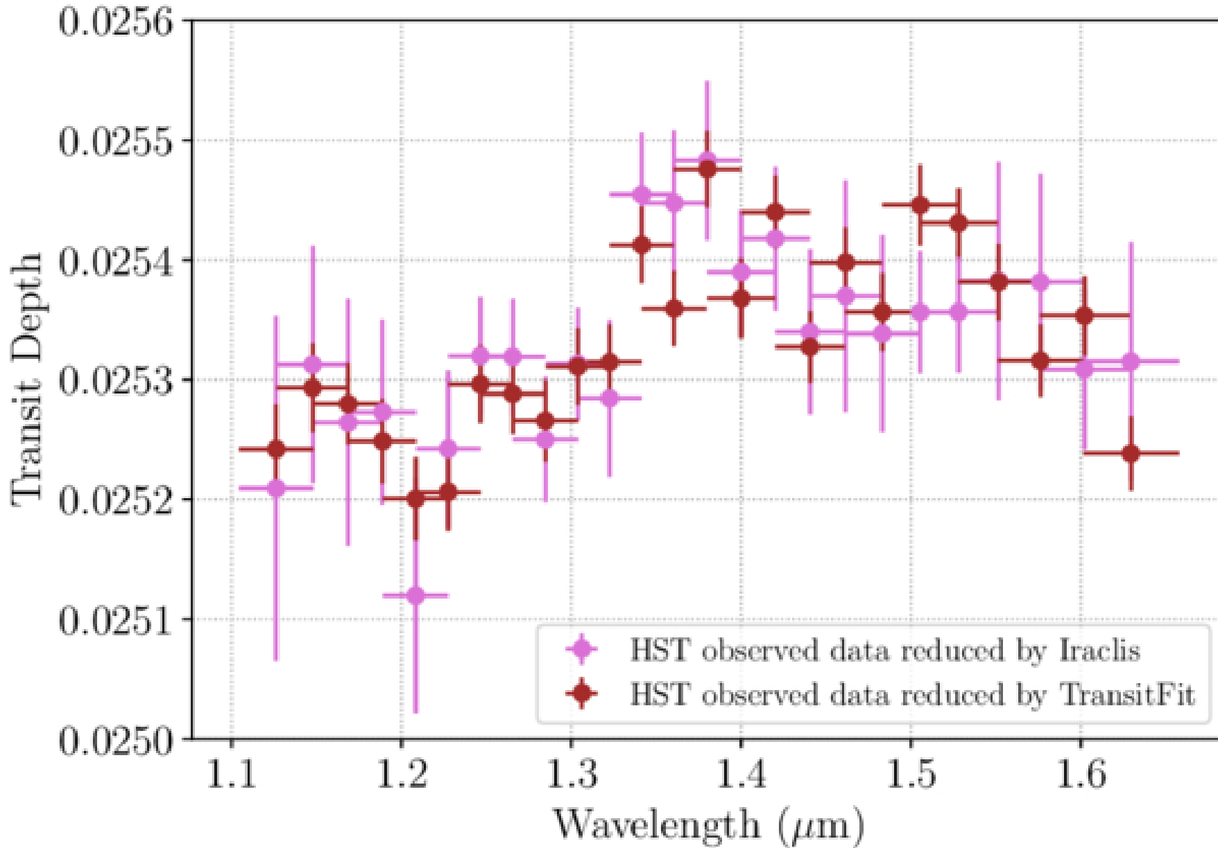
Figure 8. from Napaporn A-thano et al 2026 Astron. J. 171 doi:10.3847/1538-3881/ae5b78 https://dx.doi.org/10.3847/1538-3881/ae5b78 © 2026. The Author(s). Published by the American Astronomical Society.
