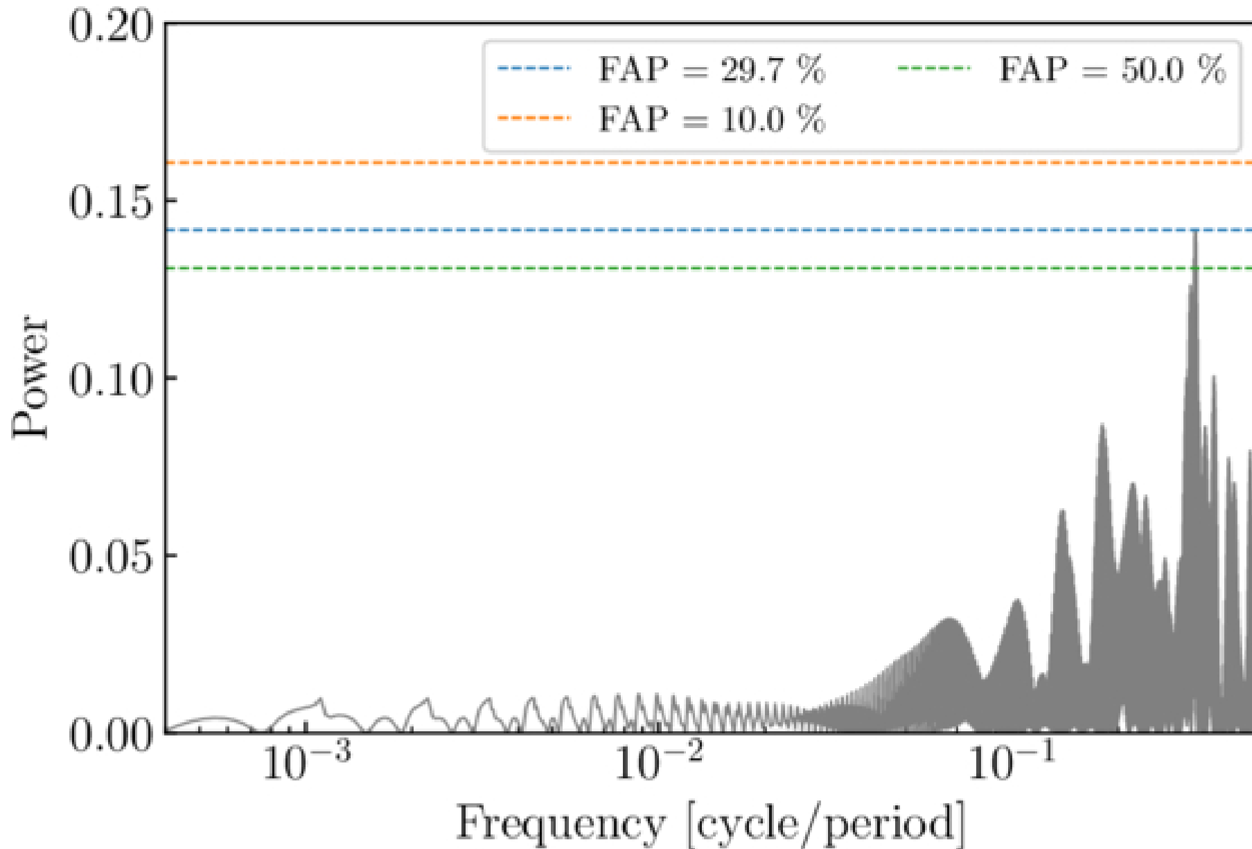
Figure 6. from Napaporn A-thano et al 2026 Astron. J. 171 doi:10.3847/1538-3881/ae5b78 https://dx.doi.org/10.3847/1538-3881/ae5b78 © 2026. The Author(s). Published by the American Astronomical Society.
