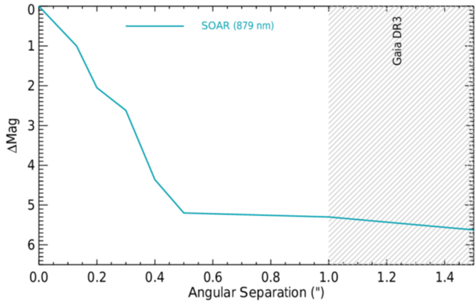
Figure 3. from Samuel N. Quinn et al 2026 Astron. J. 171 doi:10.3847/1538-3881/ae5b6a https://dx.doi.org/10.3847/1538-3881/ae5b6a © 2026. The Author(s). Published by the American Astronomical Society.
