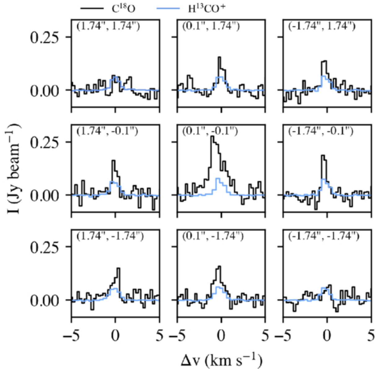
Figure 4. from K. R. Schwarz et al 2026 Astron. J. 171 doi:10.3847/1538-3881/ae5b65 https://dx.doi.org/10.3847/1538-3881/ae5b65 © 2026. The Author(s). Published by the American Astronomical Society.
