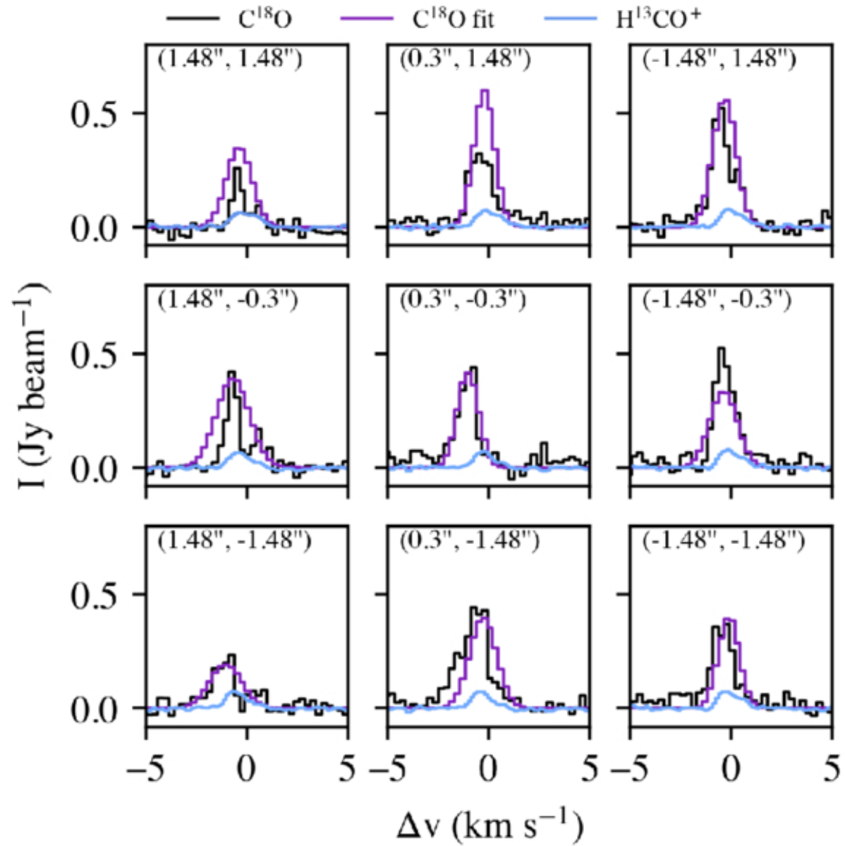
Figure 2. from K. R. Schwarz et al 2026 Astron. J. 171 doi:10.3847/1538-3881/ae5b65 https://dx.doi.org/10.3847/1538-3881/ae5b65 © 2026. The Author(s). Published by the American Astronomical Society.
